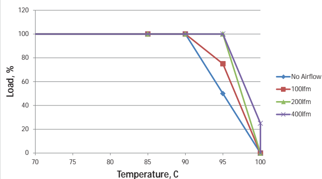
MTC1S2403MC- 18Vin
