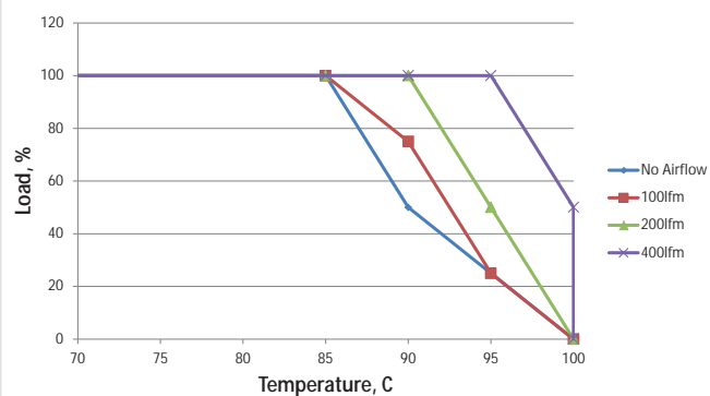
MTC1S1203MC - 9Vin
