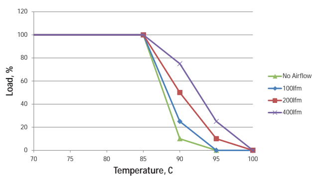
MTC1S2412MC- 36Vin
