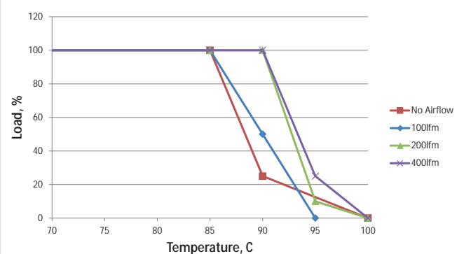
MTC1S2403MC - 24Vin
