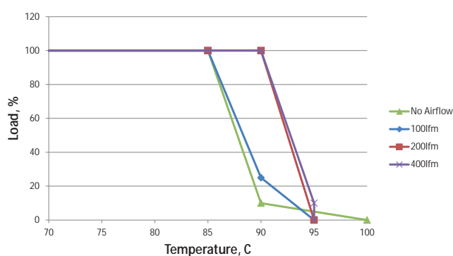
MTC1S2403MC- 36Vin
