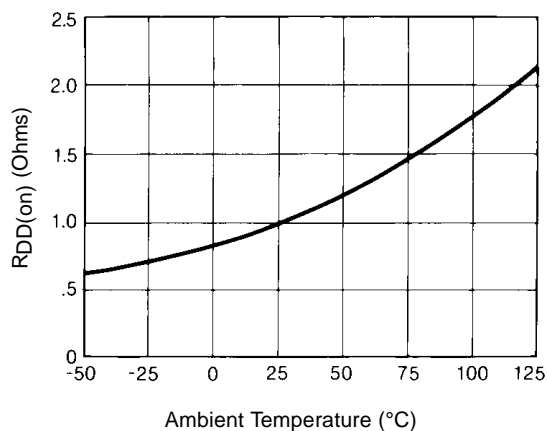
Figure 4. Typical On-Resistance
