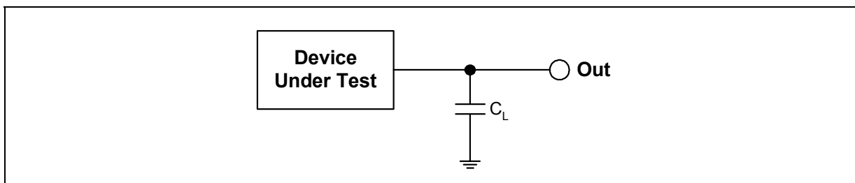
Figure 13: Transient Equivalent Testing Load Circuit
