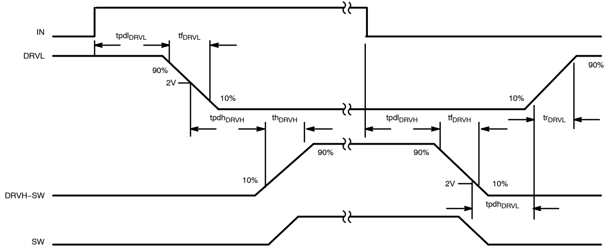
Figure 5. Timing Diagram
