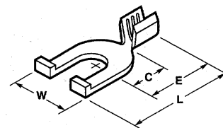
D Flanged
