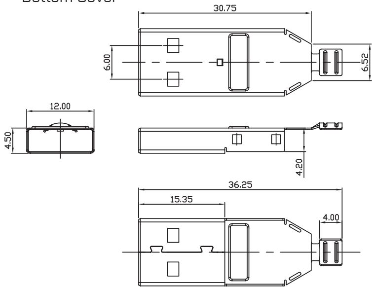
Bottom Cover
