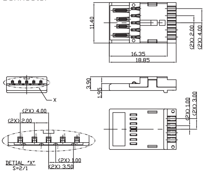
Connector
