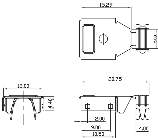
Top Cover
