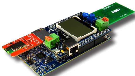
NXP/Zentri LPC43S67-A70CM Cloud Connectivity Kit (P/N OM13086)
