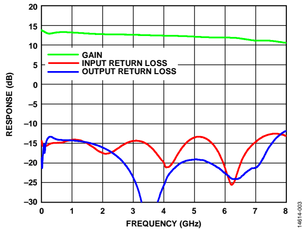
Figure 3. Response (Gain, Input Return Loss, and Output Return Loss) vs. Frequency (Linear Scale)
