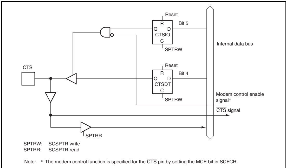
Figure 15.20 CTSIO Bit, CTSDT Bit, and \overline{\text{CTS}} Pin
