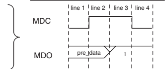
Example of corresponding waveforms
