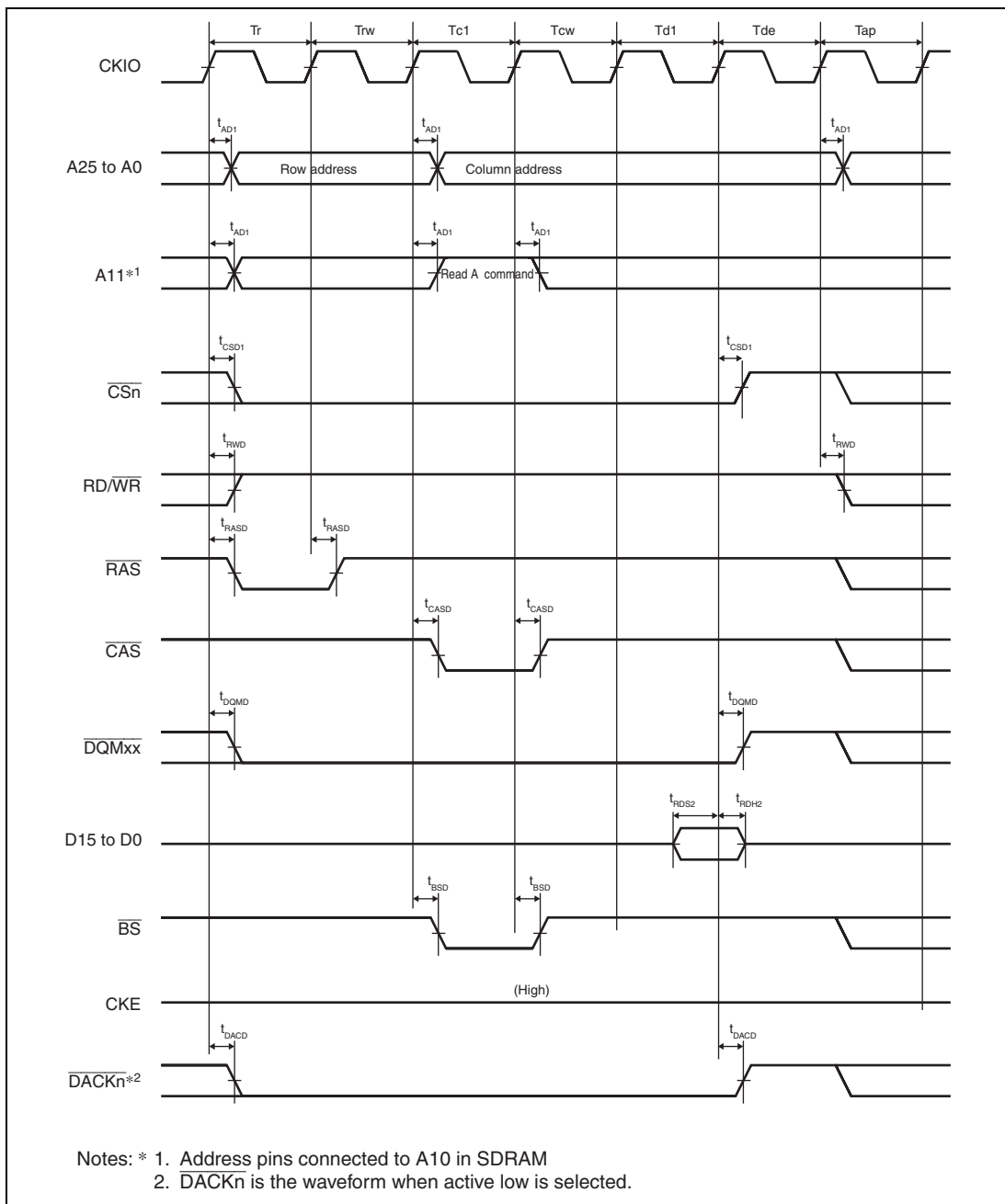
Figure 25.17 Synchronous DRAM Single Read Bus Cycle (Auto-Precharge, CAS Latency = 2, WTRCD = 1 Cycle, WTRP = 1 Cycle)
