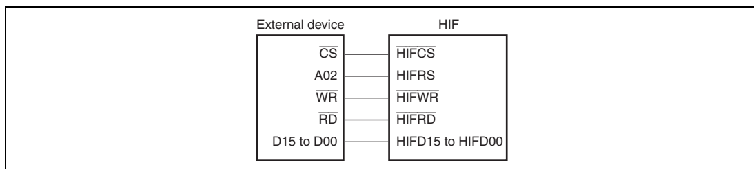
Figure 17.2 HIF Connection Example
