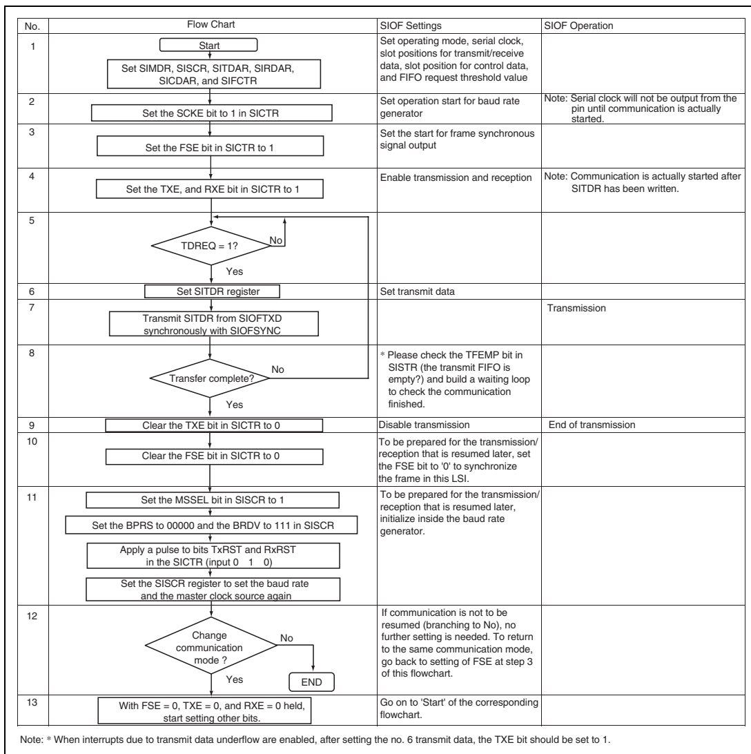
Figure 16.9 (2) Transmission Operation in Master Mode (Example of Half-Duplex Transmission by the CPU with TDMAE=0)
