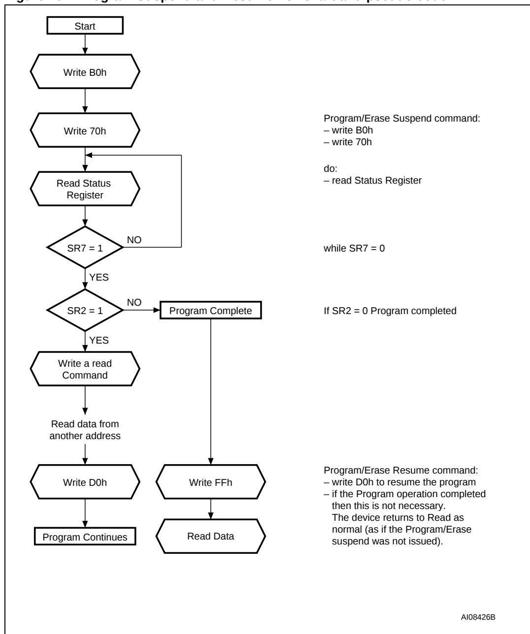
Figure 20. Program Suspend and Resume flowchart and pseudo code
