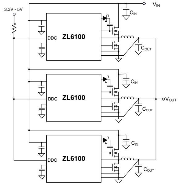
FIGURE 21. CURRENT SHARING GROUP
