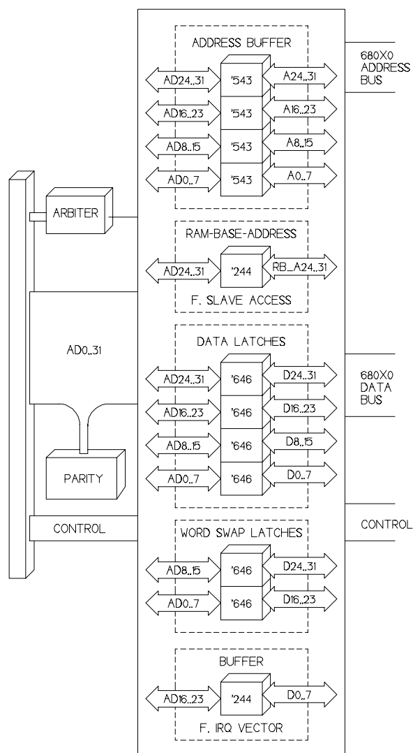
Figure 5. Sample Interface
