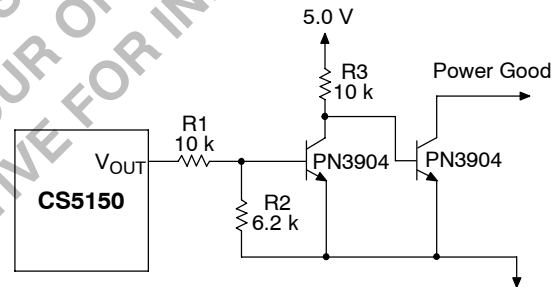
Figure 17. Implementing Power Good with the CS5150
