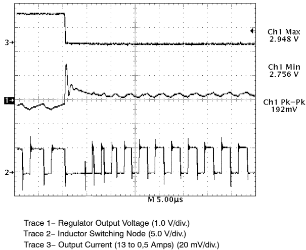
Figure 11. CS5150 Demonstration Board Response to 13 A Load Turn Off (Output Set for 2.8 V). V^2 Control Topology Immediately Connects Inductor to Ground, Providing 0% Duty Cycle. Regulation is Achieved in Less Than 10 \mu s
