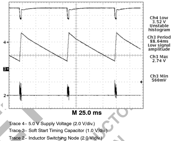
Figure 12. CS5150 Demonstration Board Hiccup Mode Short Circuit Protection. Gate Pulses are Delivered While the Soft Start Capacitor Charges, and Cease During Discharge
