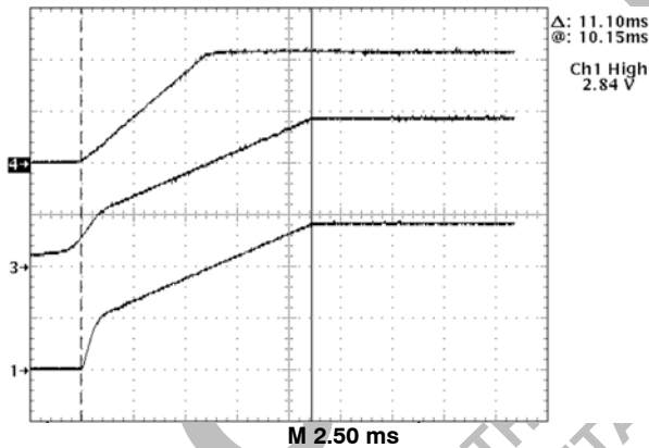
Figure 4. CS5150 Demonstration Board Startup in Response to Increasing 12 V and 5.0 V Input Voltages. Extended Off Time is Followed by Normal Off Time Operation when Output Voltage Achieves Regulation to the Error Amplifier Output.
