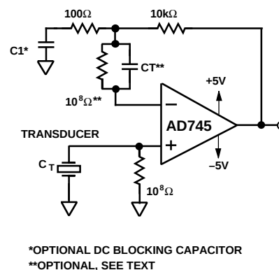
Figure 34. A Piezoelectric Transducer
