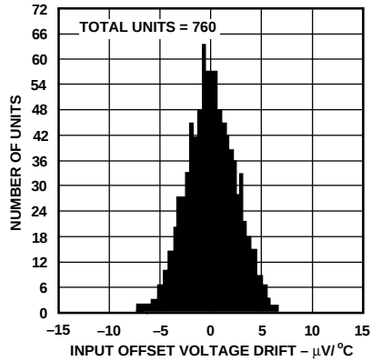
Figure 19. Distribution of Offset Voltage Drift. T_A = +25^\circ\text{C} to +125^\circ\text{C}
