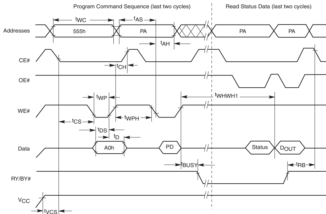
Figure 15.5 Program Operation Timings
