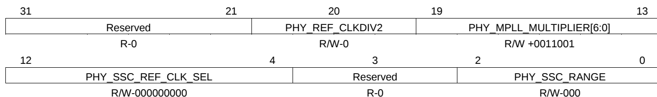
Figure 9-42. USB_PHY_CTL5 Register
