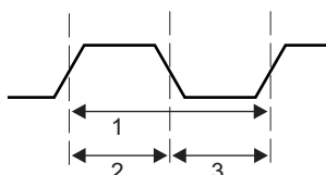
Figure 11-36. HyperLink Station Management Clock Timing
