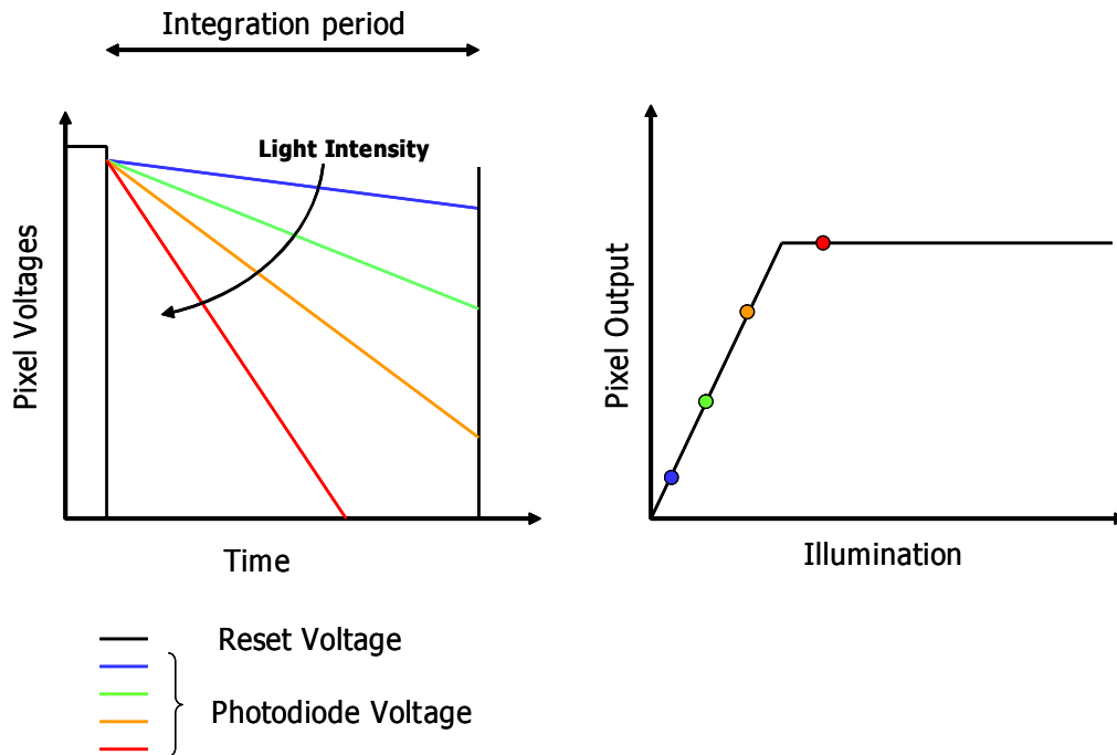
Figure 9. Left: Sketch of photodiode pixel voltage vs. time showing how different light intensities affect this parameter. Right: Sketch of the corresponding sensor ADC output vs illumination. The response is linear with an eventual saturation.
