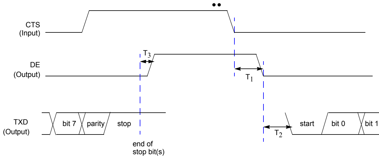
Figure 77. UART Timing With CTS
