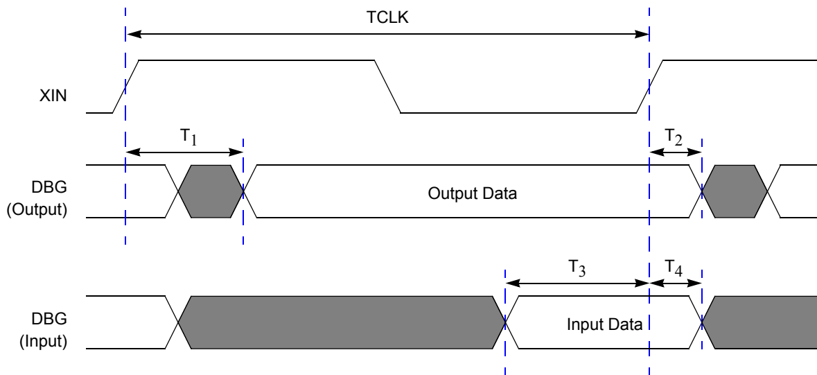
Figure 76. On-Chip Debugger Timing
