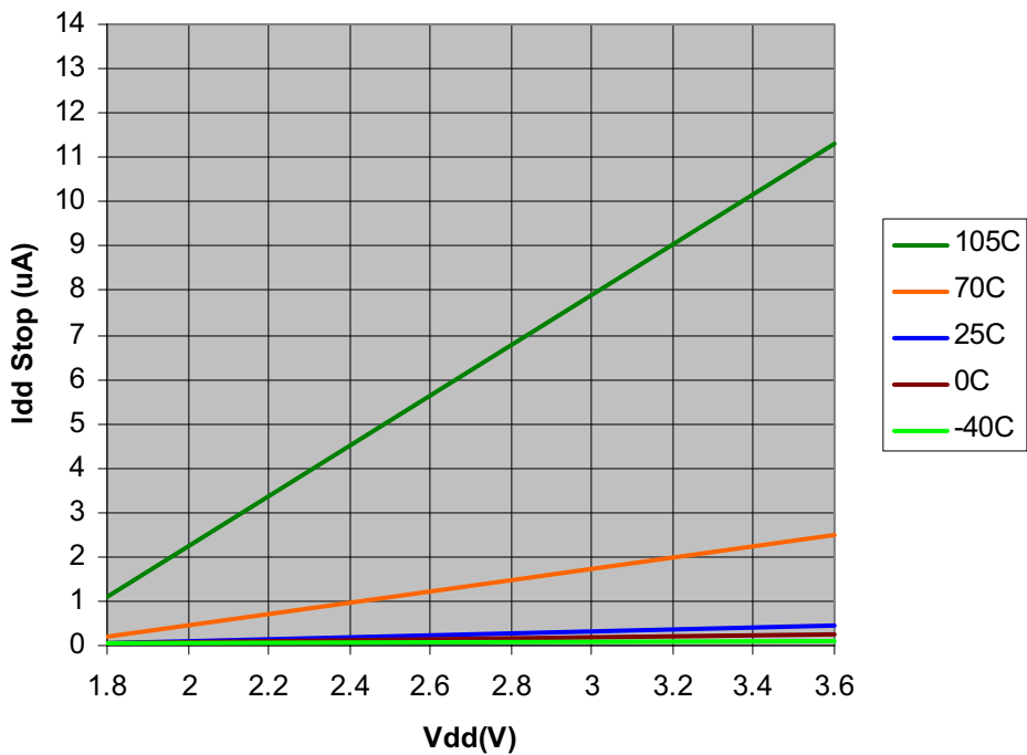
Figure 72. STOP Mode Current Consumption as a Function Vdd with Temperature as a Parameter— All Peripheral Disabled
