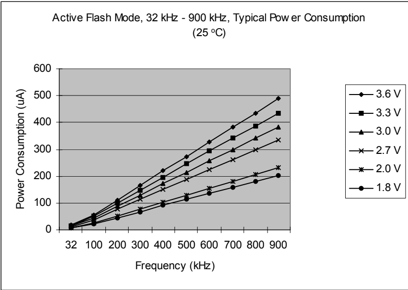
Figure 70. Typical Active Flash Mode Supply Current (32 – 900 kHz)
