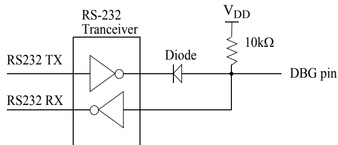
Figure 56. Interfacing the On-Chip Debugger's DBG Pin with an RS-232 Interface (1)
