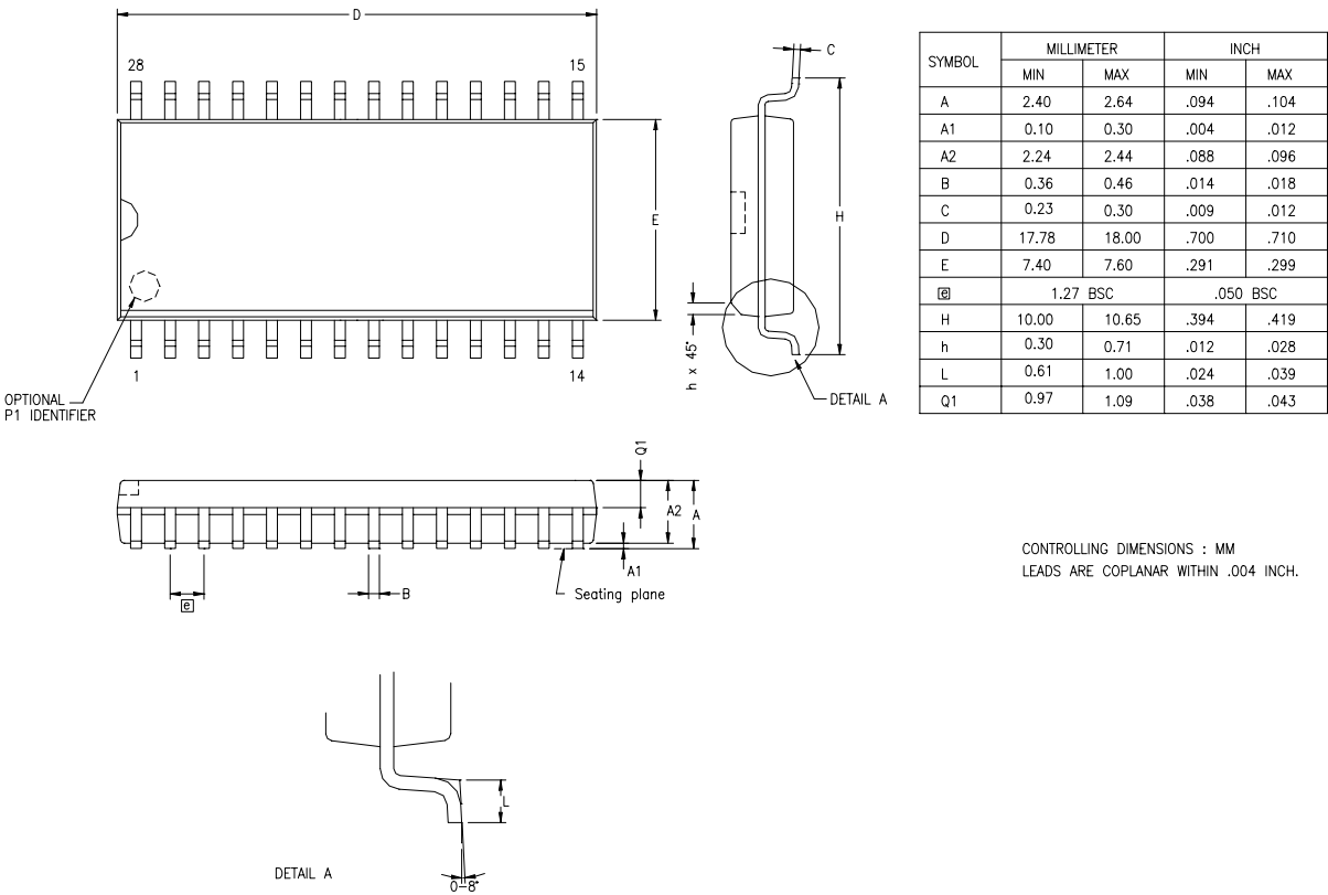
Figure 82. 28-Pin Small Outline Integrated Circuit Package (SOIC)
