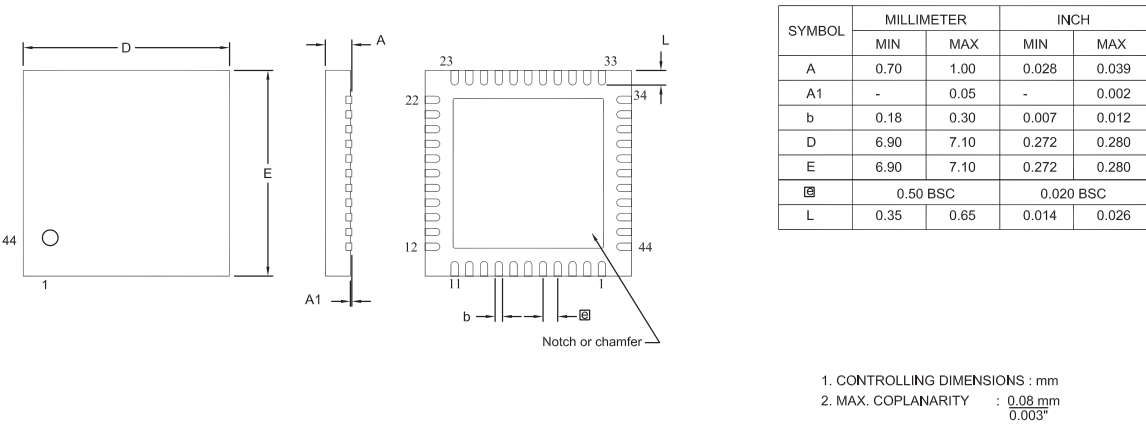
Figure 86. 44-Lead Quad Flat No Lead Package (QFN)
