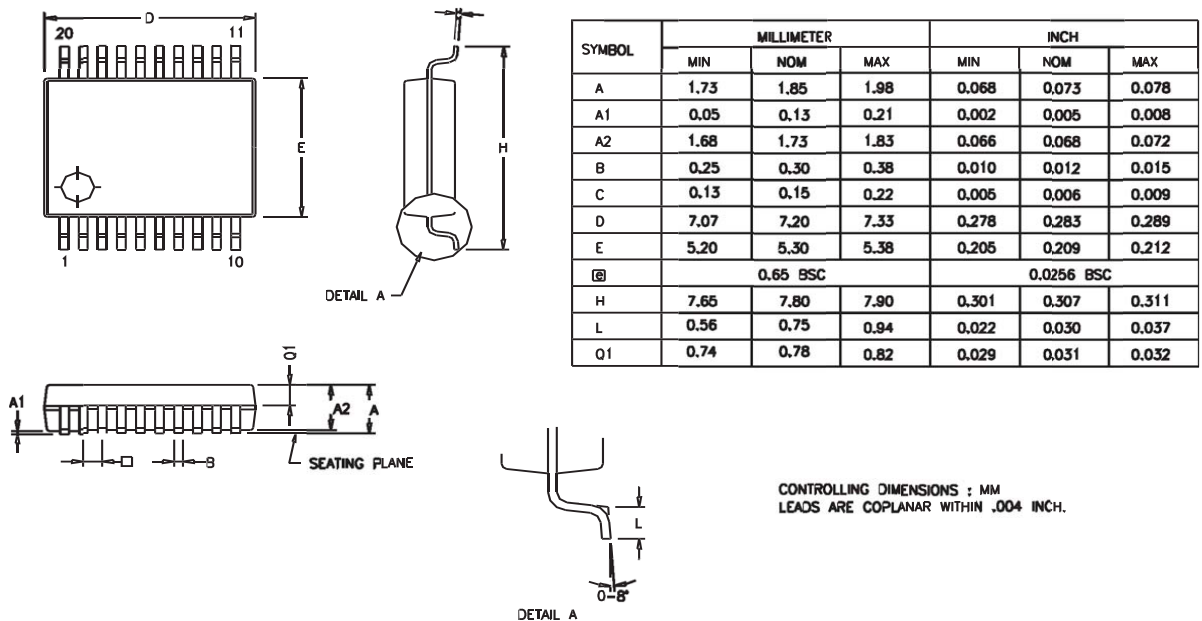
Figure 80. 20-Pin Small Shrink Outline Package (SSOP)
