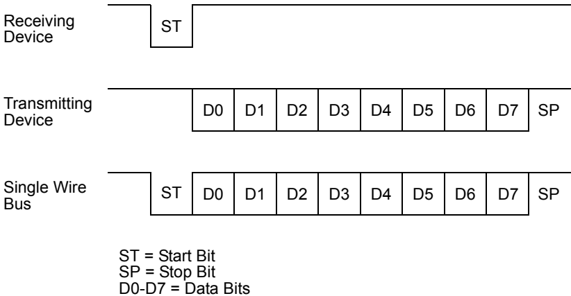
Figure 60. Start Bit Flow Control
