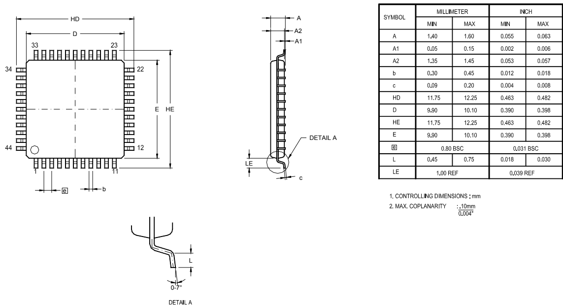
Figure 85. 44-Lead Low-Profile Quad Flat Package (LQFP)
