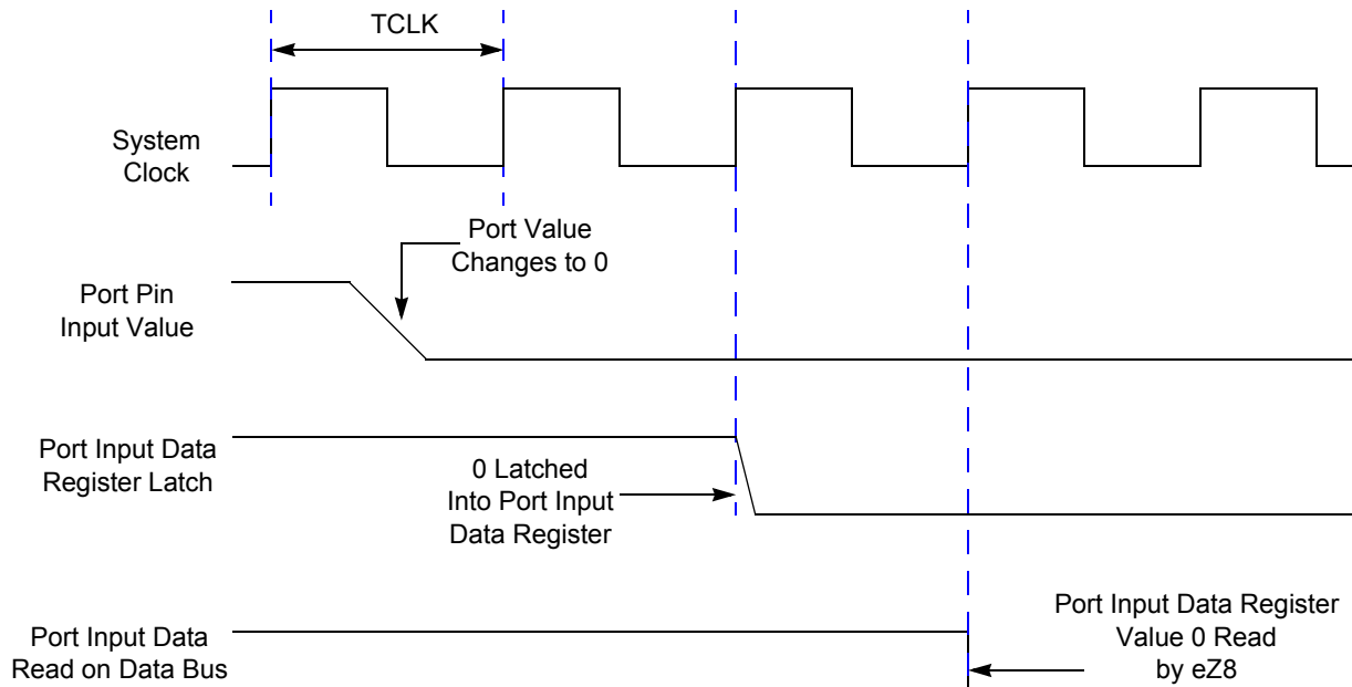
Figure 74. Port Input Sample Timing
