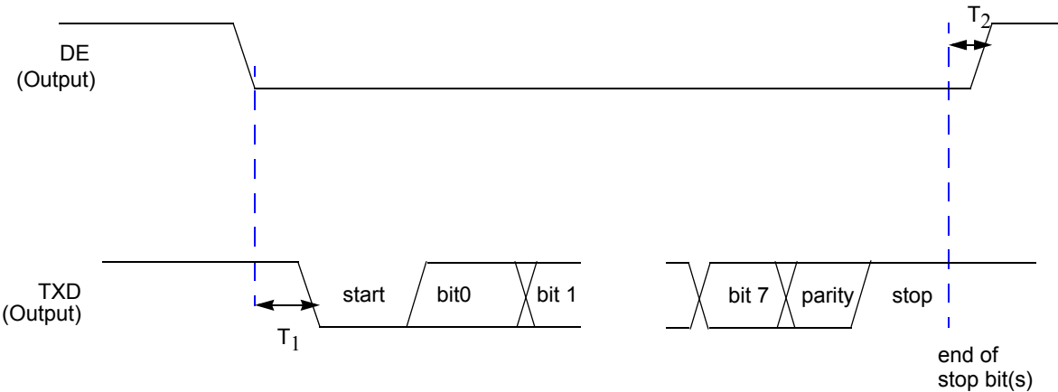
Figure 78. UART Timing Without CTS
