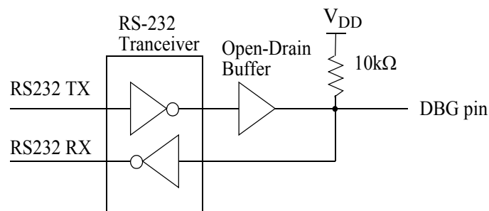
Figure 57. Interfacing the On-Chip Debugger's DBG Pin with an RS-232 Interface (2)
