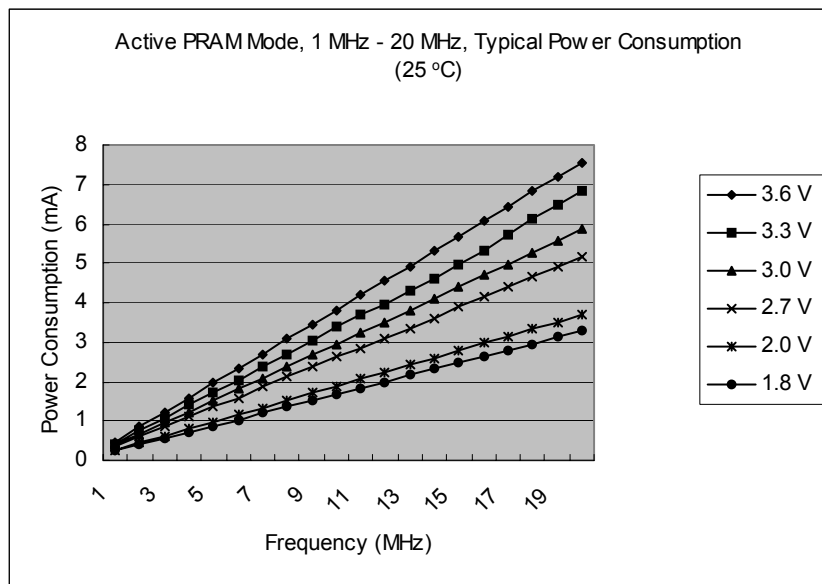
Figure 69. Typical Active PRAM Mode Supply Current (1 – 20 MHz)
