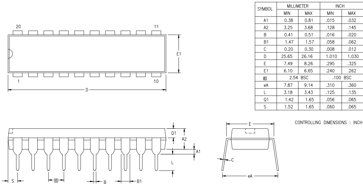
Figure 78. 20-Pin Plastic Dual Inline Package (PDIP)
