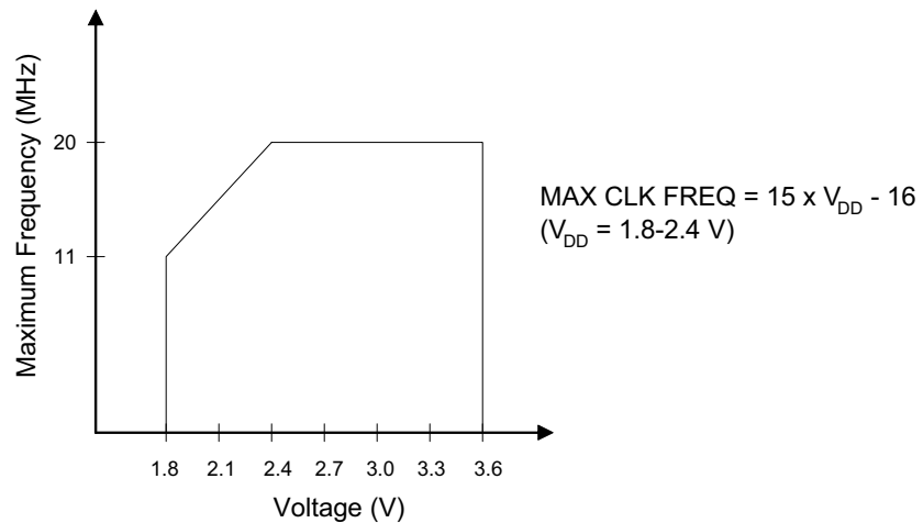
Figure 73. V_{DD} Versus Maximum System Clock Frequency
