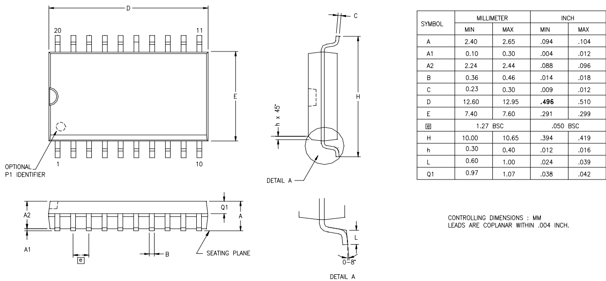
Figure 79. 20-Pin Small Outline Integrated Circuit Package (SOIC)
