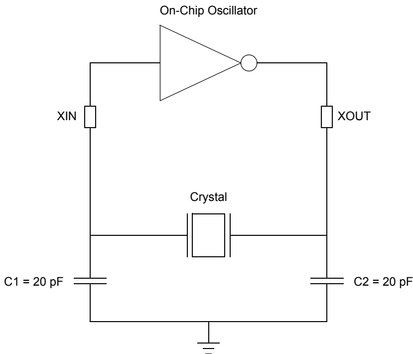
Figure 61. Recommended 20 MHz Crystal Oscillator Configuration
