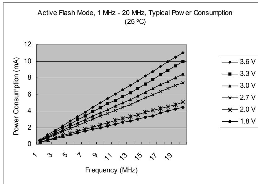
Figure 68. Typical Active Flash Mode Supply Current (1 – 20 MHz)
