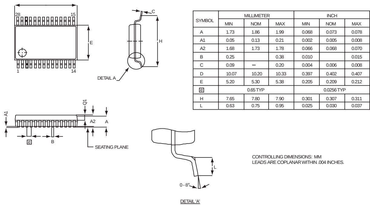
Figure 83 illustrates the 28-pin Small Shrink Outline Package (SSOP) available for the Z8 Encore! XP F1680 Series devices.
