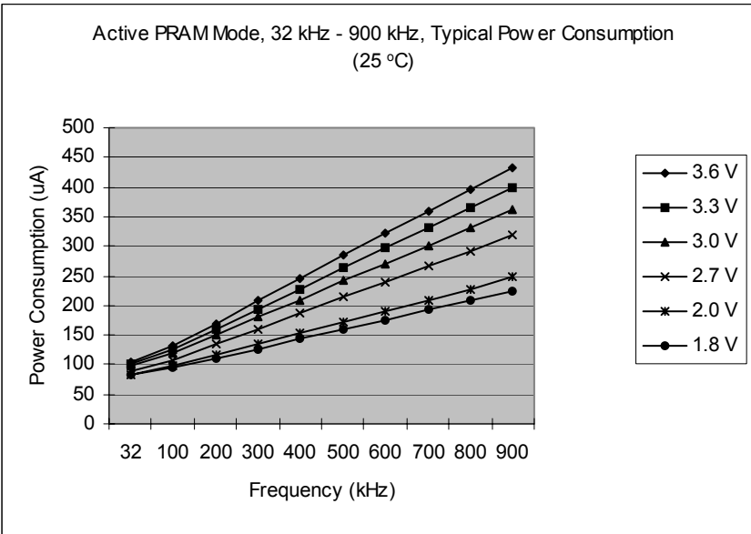
Figure 71. Typical Active PRAM Mode Supply Current (32–900 kHz)
