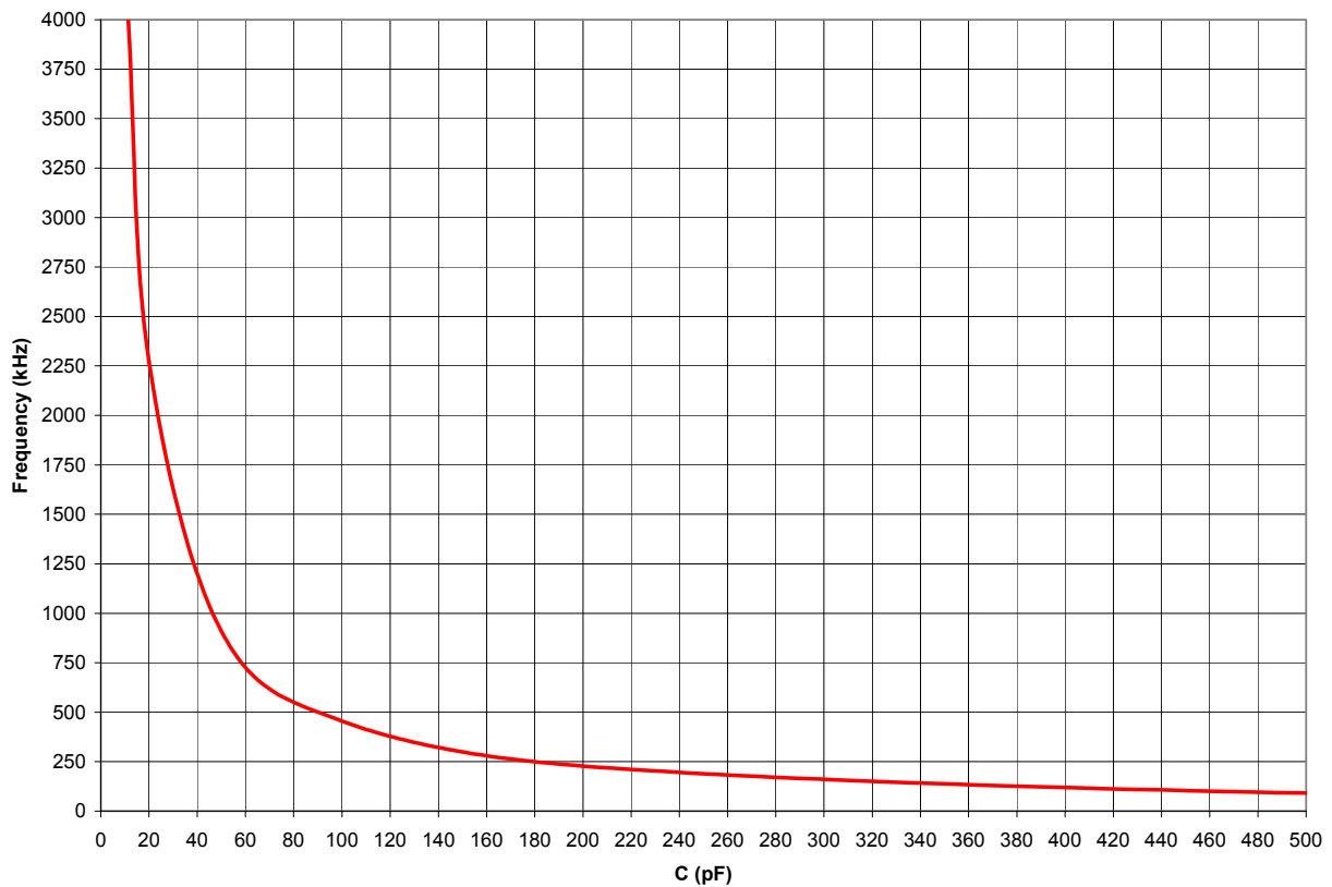
Figure 63. Typical RC Oscillator Frequency as a Function of the External Capacitance with a 45 K \Omega Resistor
