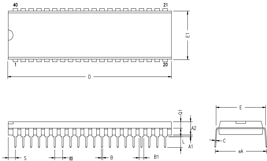
Figure 84. 40-Lead Plastic Dual-Inline Package (PDIP)
