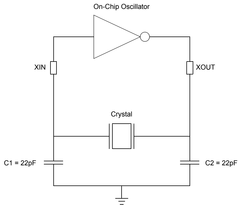
Figure 64. Recommended 32 kHz Crystal Oscillator Configuration
