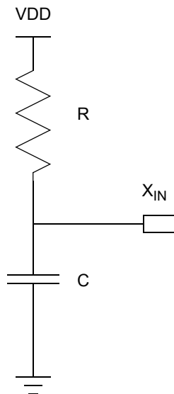
Figure 62. Connecting the On-Chip Oscillator to an External RC Network
