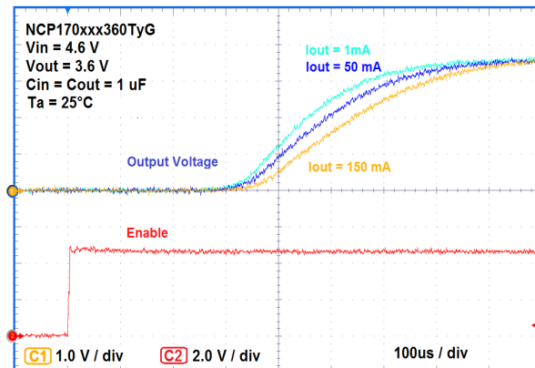
Figure 48. Enable Turn-on Response at V_{out} = 3.6\text{ V}
