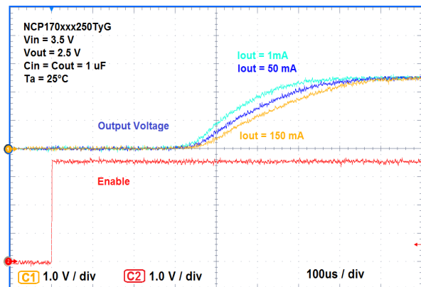
Figure 47. Enable Turn-on Response at V_{out} = 2.5\text{ V}
