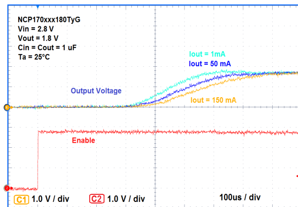
Figure 46. Enable Turn-on Response at V_{out} = 1.8\text{ V}
