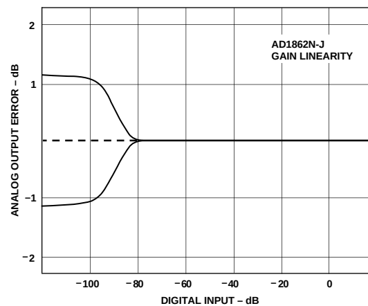
Figure 4. Gain Linearity
