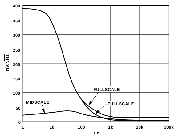
Figure 2. Noise Density
