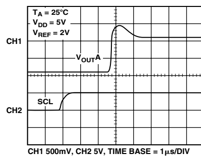
Figure 21. Exiting Power-Down to Midscale
