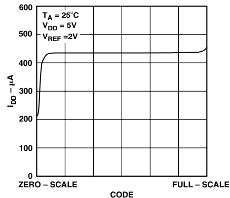
Figure 15. Supply Current vs. DAC Code
