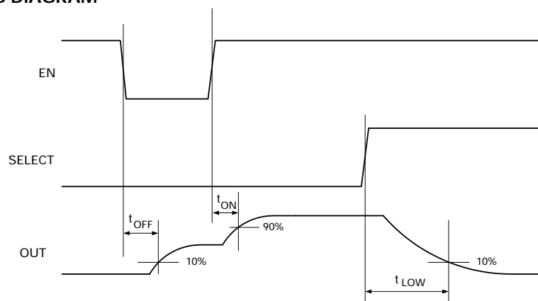
Fig.2: TIMING DIAGRAM
