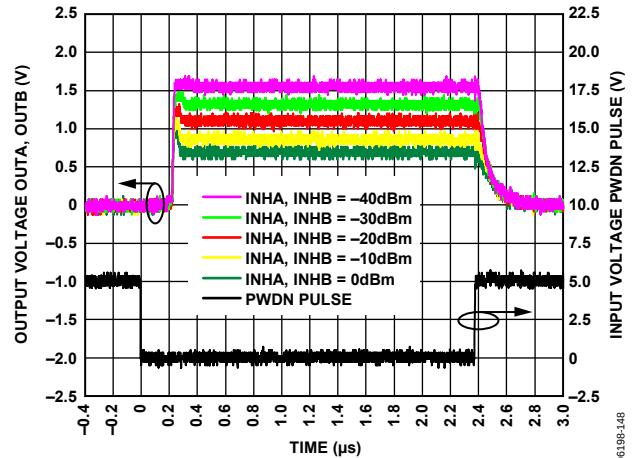
Figure 48. Output Response Using Power-Down Mode for Various RF Input Levels, Carrier Frequency = 900 MHz, CLPA = 0.1 \mu F
