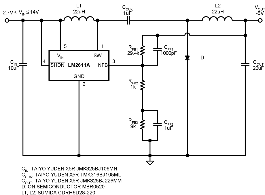
FIGURE 16. LM2611 High Current Schematic
