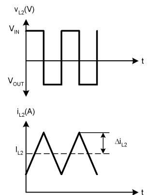
FIGURE 3. Voltage and Current Waveforms in Inductor L2 of a Cuk Converter
