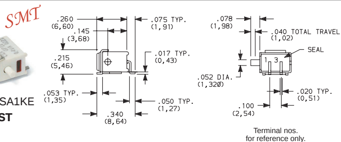
PC MOUNTING
