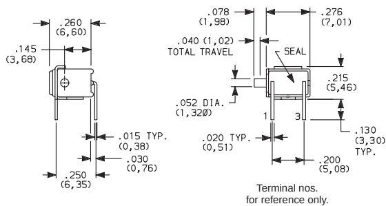
PC MOUNTING
