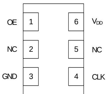
Si530 CMOS
