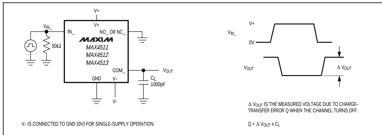
Figure 4. Charge Injection
