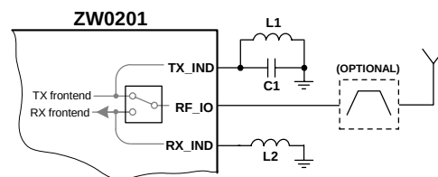
Figure 7: RF interface in typical application
