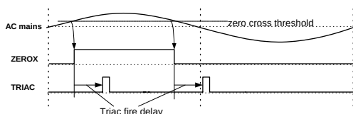
Figure 16: View of triac waveforms with exaggerated zero cross detection offset
