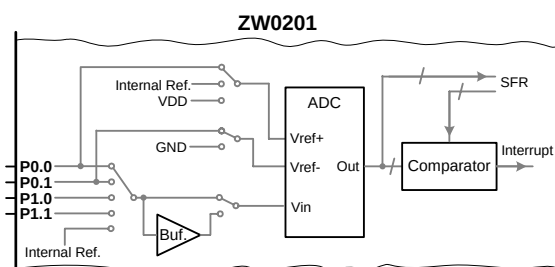
Figure 18: ADC block
