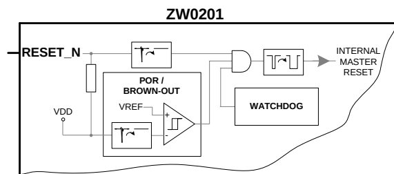
Figure 6: Reset interface
