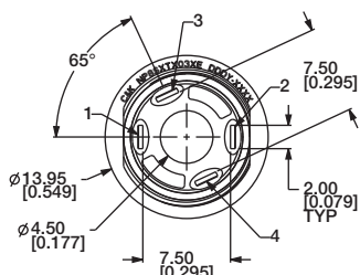
ACROSS FLATS
