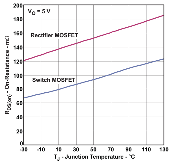
Figure 24. MOSFET r_{DS(on)} vs Temperature
