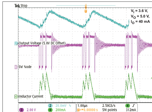
Figure 29. Power-Save Mode Operation
