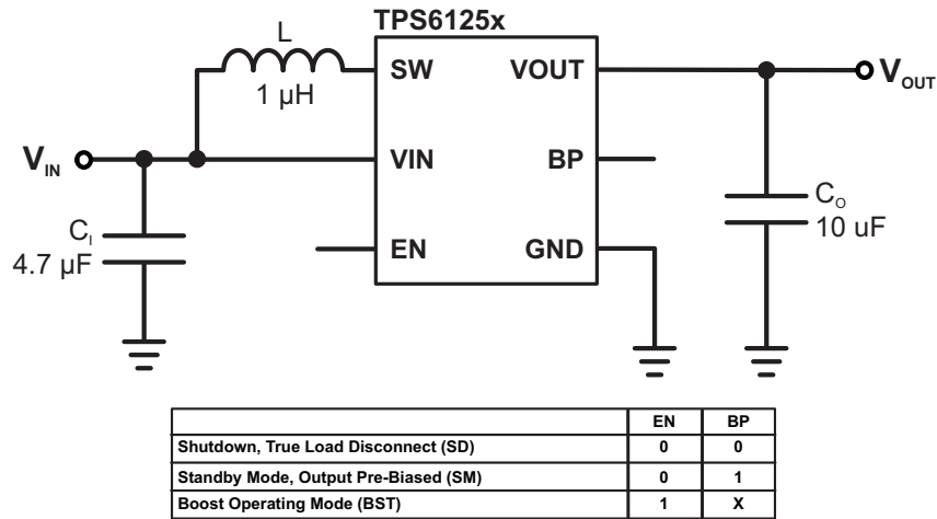
Figure 25. Parameter Measurement Schematic
