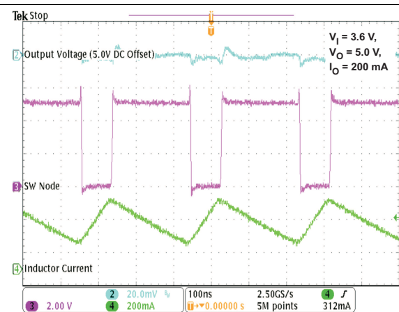
Figure 30. PWM Operation
