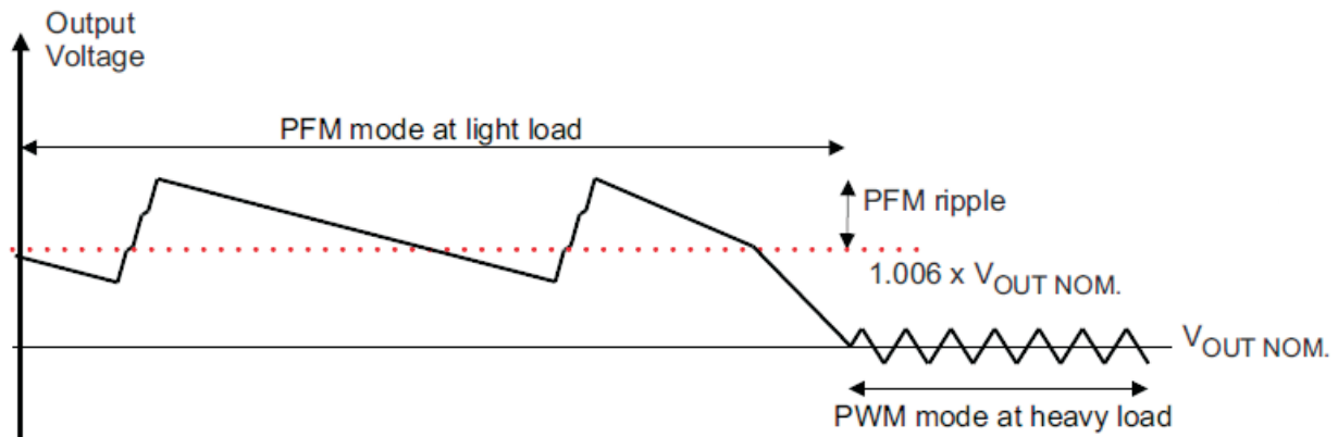
Figure 27. Power Save
