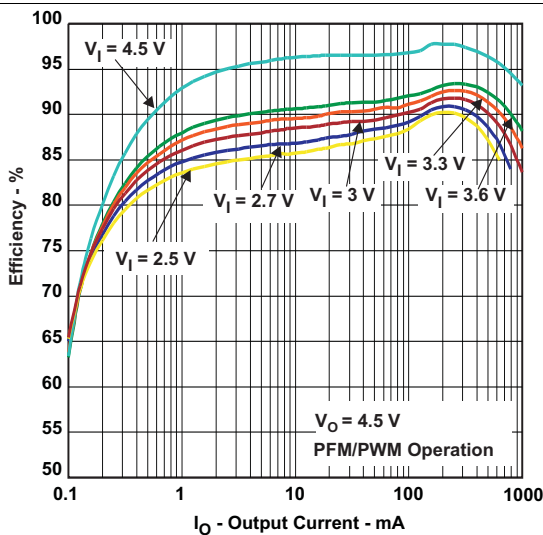
Figure 1. Efficiency vs Output Current
