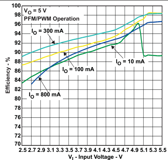
Figure 4. Efficiency vs Input Voltage
