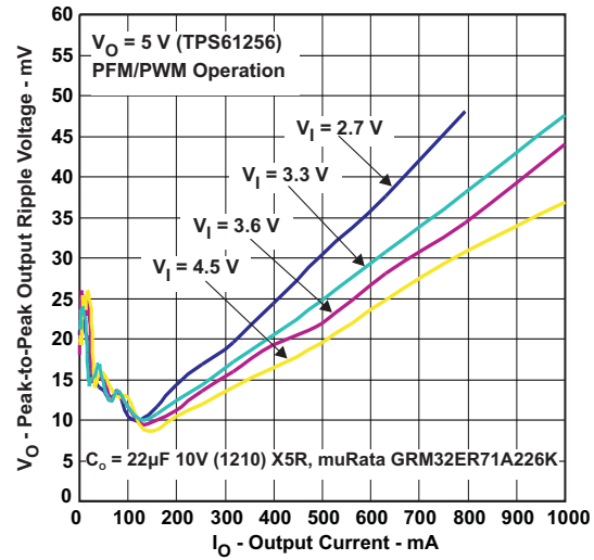
Figure 16. Peak-to-Peak Output Ripple Voltage vs Output Current
