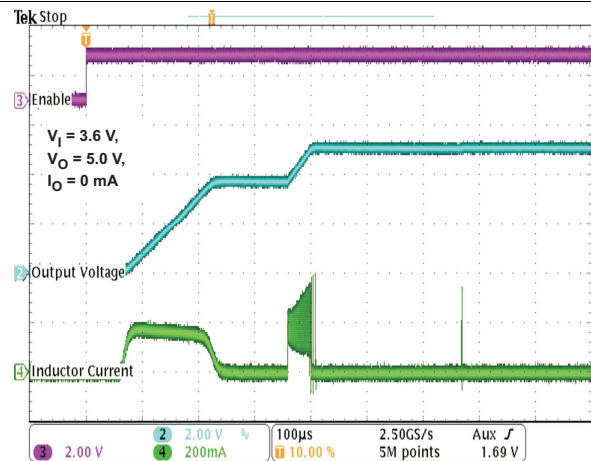
Figure 36. Start-Up
