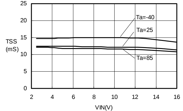
TSS-VIN S-8520/21(Fosc:60kHz)
