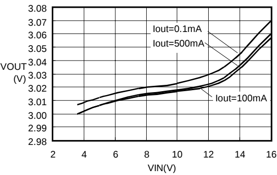
VOUT-VIN S-8521B30MC (Ta=25°C)
