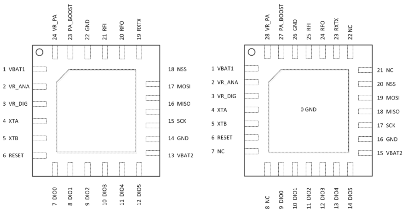
Figure 2. Pin Diagram SX1232 & SX1232B
