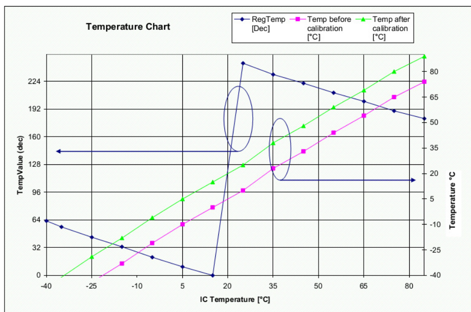
Figure 13. Temperature Sensor Response
