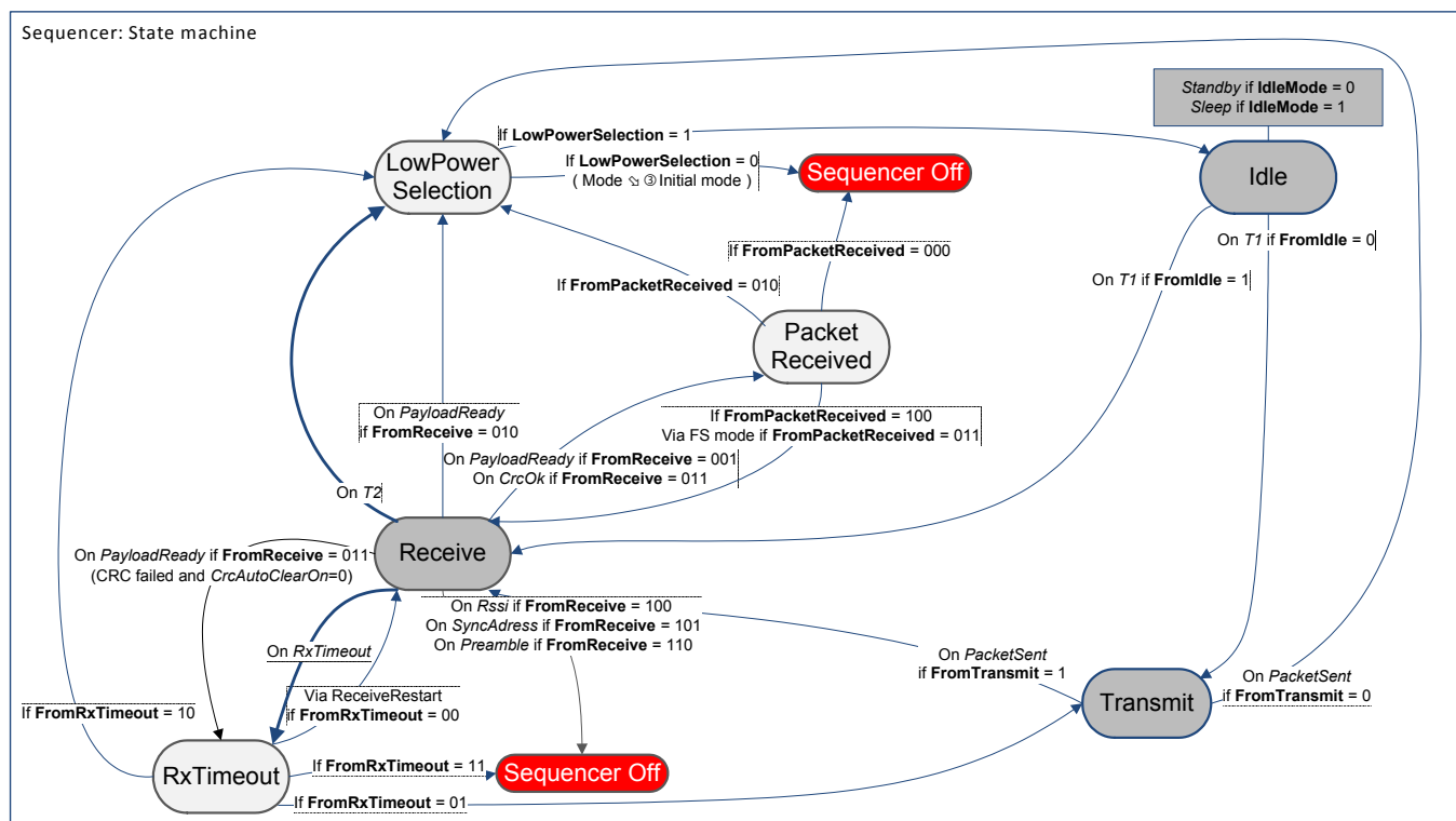
Figure 21. Sequencer State Machine
