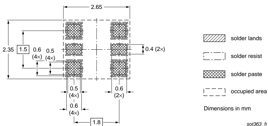
Fig 13. Reflow soldering footprint PUMB9 (SOT363)
