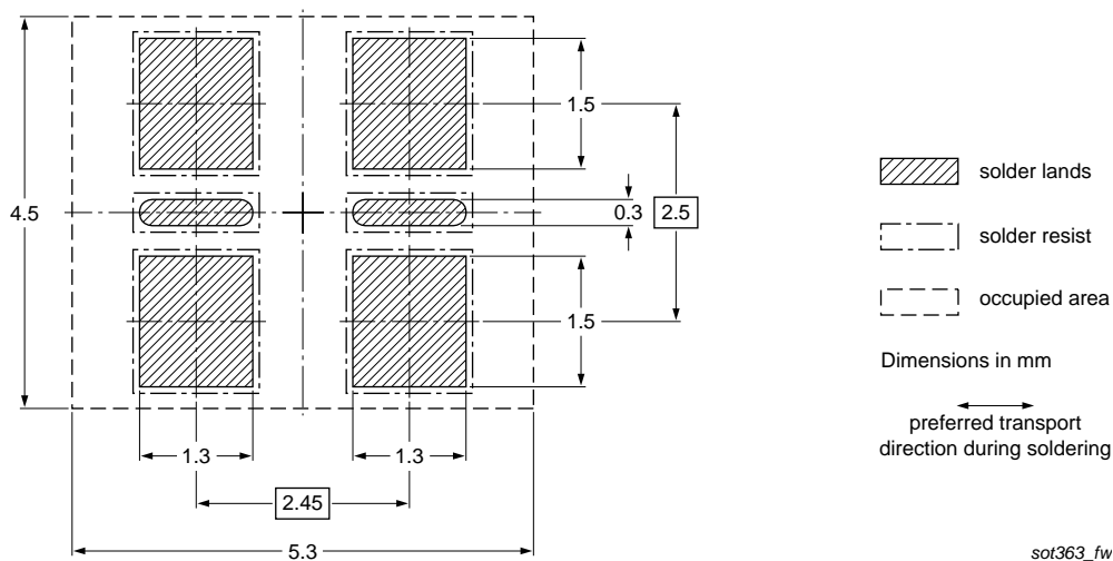
Fig 14. Wave soldering footprint PUMB9 (SOT363)
