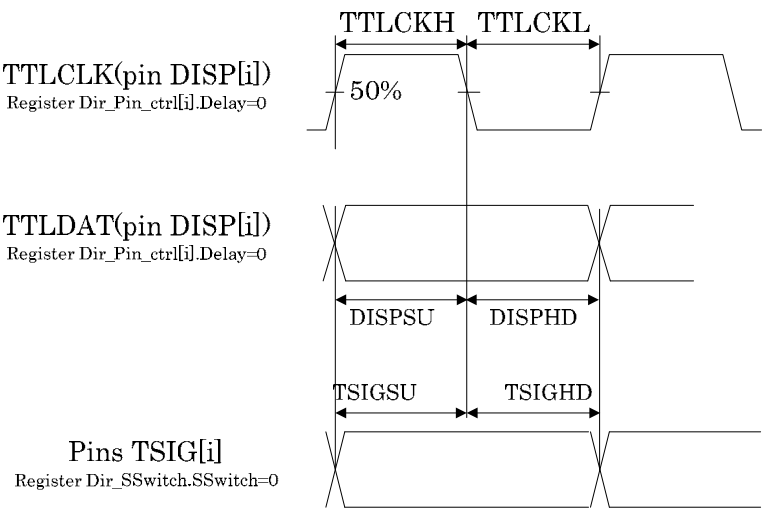
Figure 32-12 TTL operation output timing (not bypass mode) (1)
