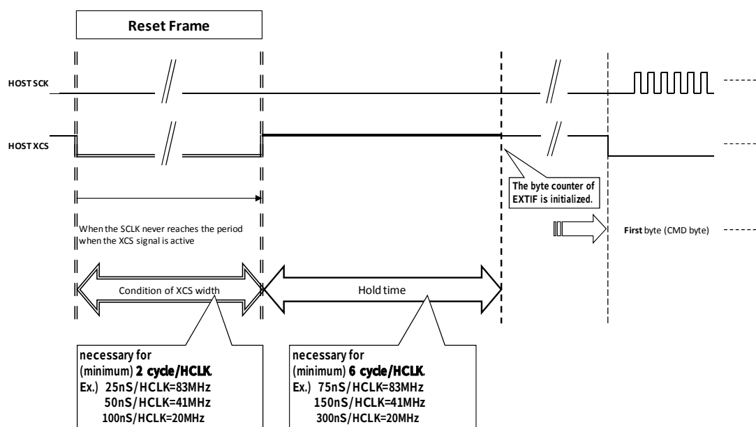
Figure 4-10 Reset Frame
