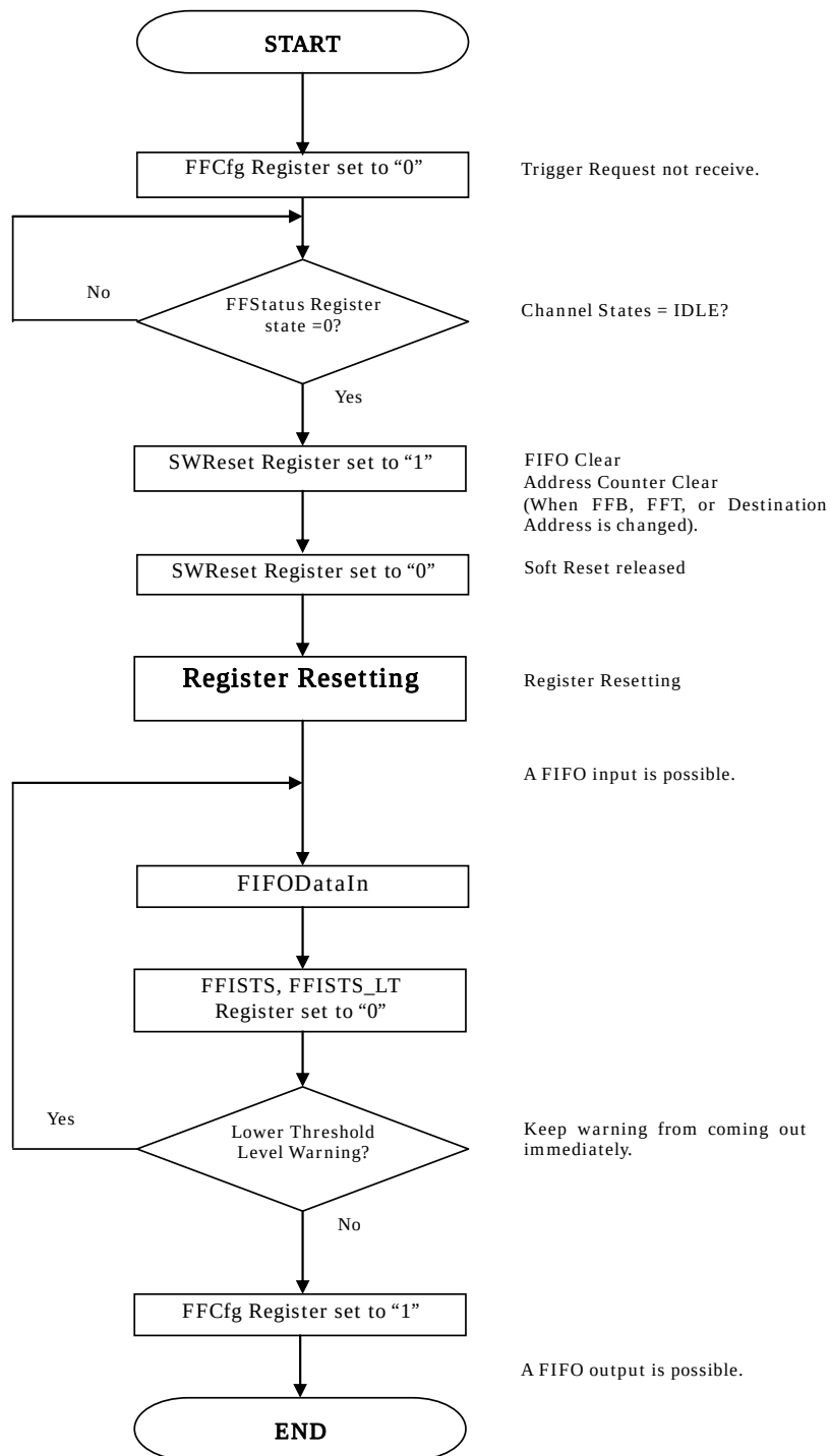
Figure 22-10 Register Resetting Flow
