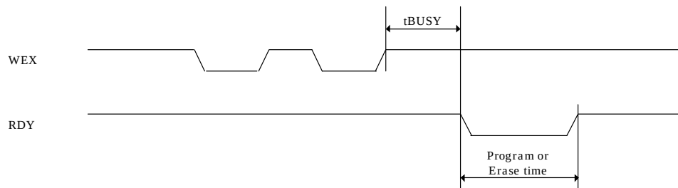
Figure 15.6-3 Program/Erase characteristics
