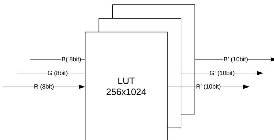
Figure 11-1 CLUT Input/Output
