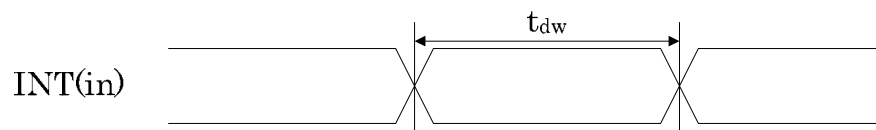
Figure 32-6 External Interrupt Timings
