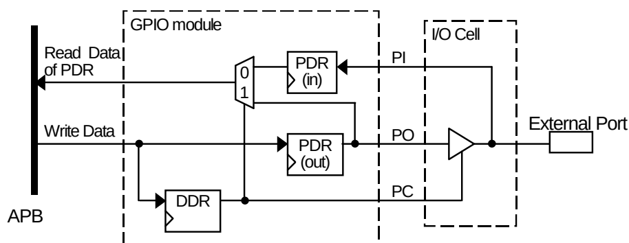
Figure 27-1 GPIO interface basic block block diagram
