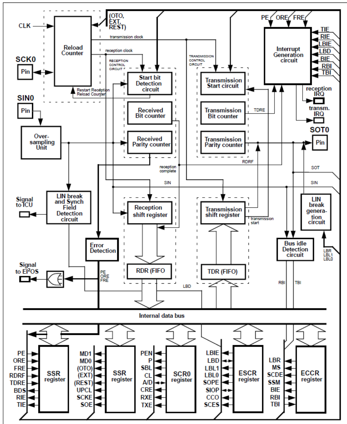
Figure 26-1 Block Diagram
