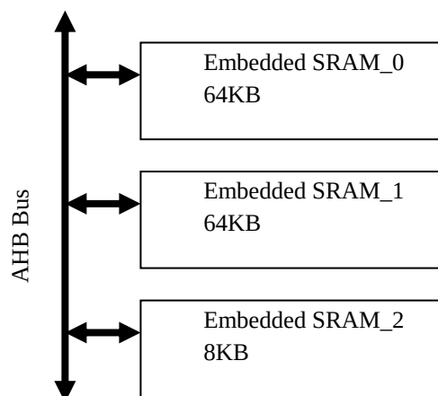
Figure 16-1 Block diagram of Internal SRAM
