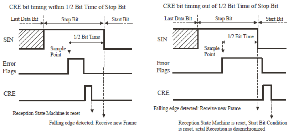
Figure 26-26 Timing of the CRE bit
