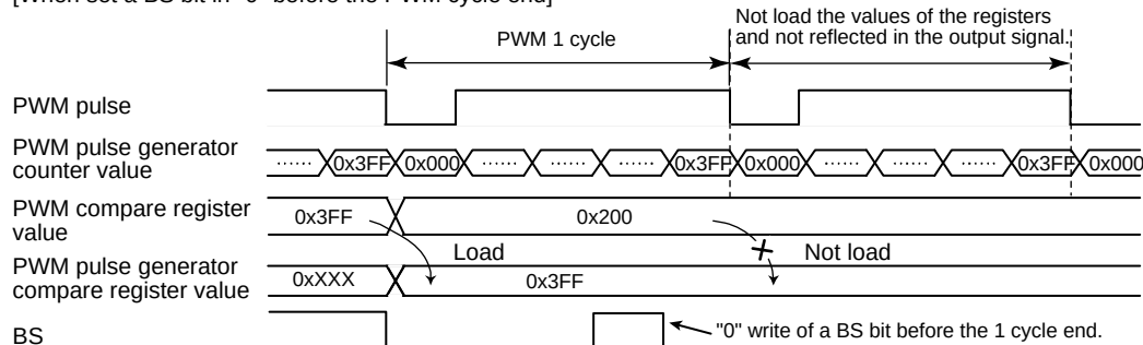
Figure 23-4 load timing of PWM compare register value
