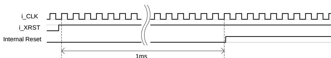
Figure 19-3 PLL stable waiting period timing diagram
