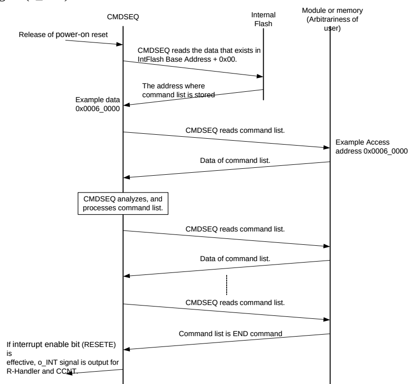
Figure 7.3-2 Reset start
