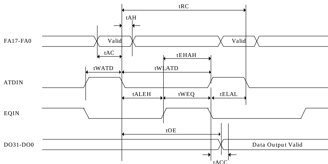
Figure 15.6-1 Synchronous Read
