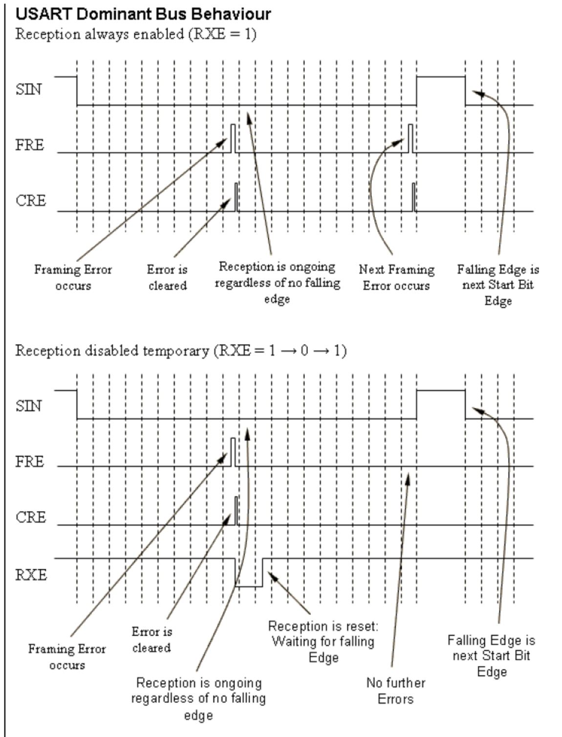
Figure 26-28 USART Dominant Bus Behaviour
