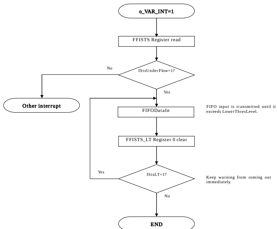
Figure 22-12 FIFO Empty Flow
