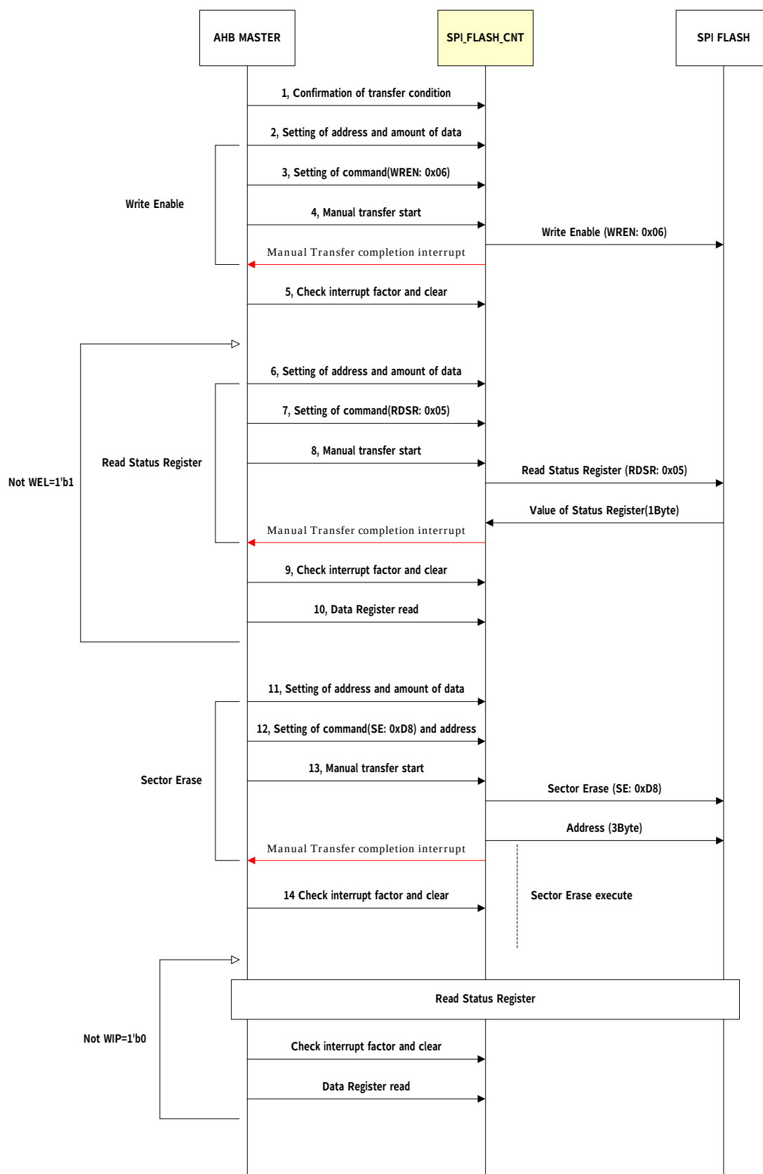
Figure 14-5 Manual Sector Erase flow
