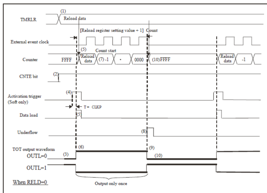
Figure 31-9 Operation in external event clock one-shot mode, (one-shot pulse is output)
