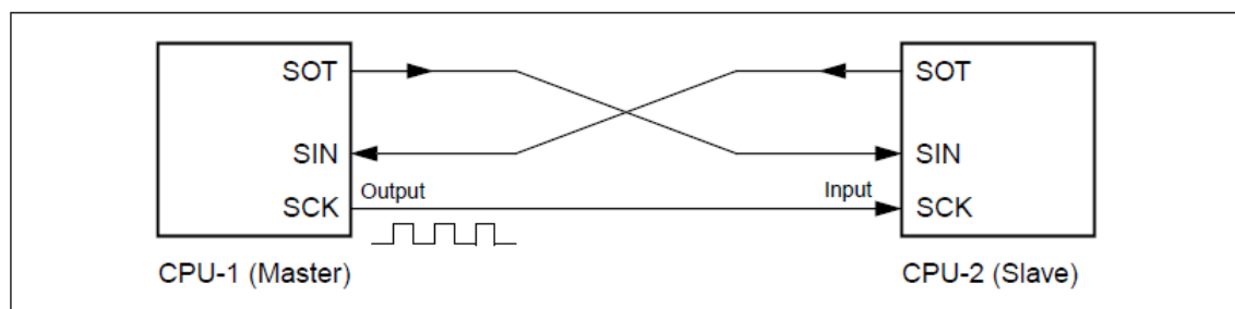
Figure 26-17 Connection example of USART mode 2 bidirectional communication
