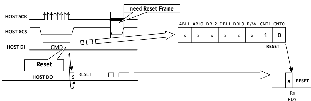
Figure 4-19 Reset Request
