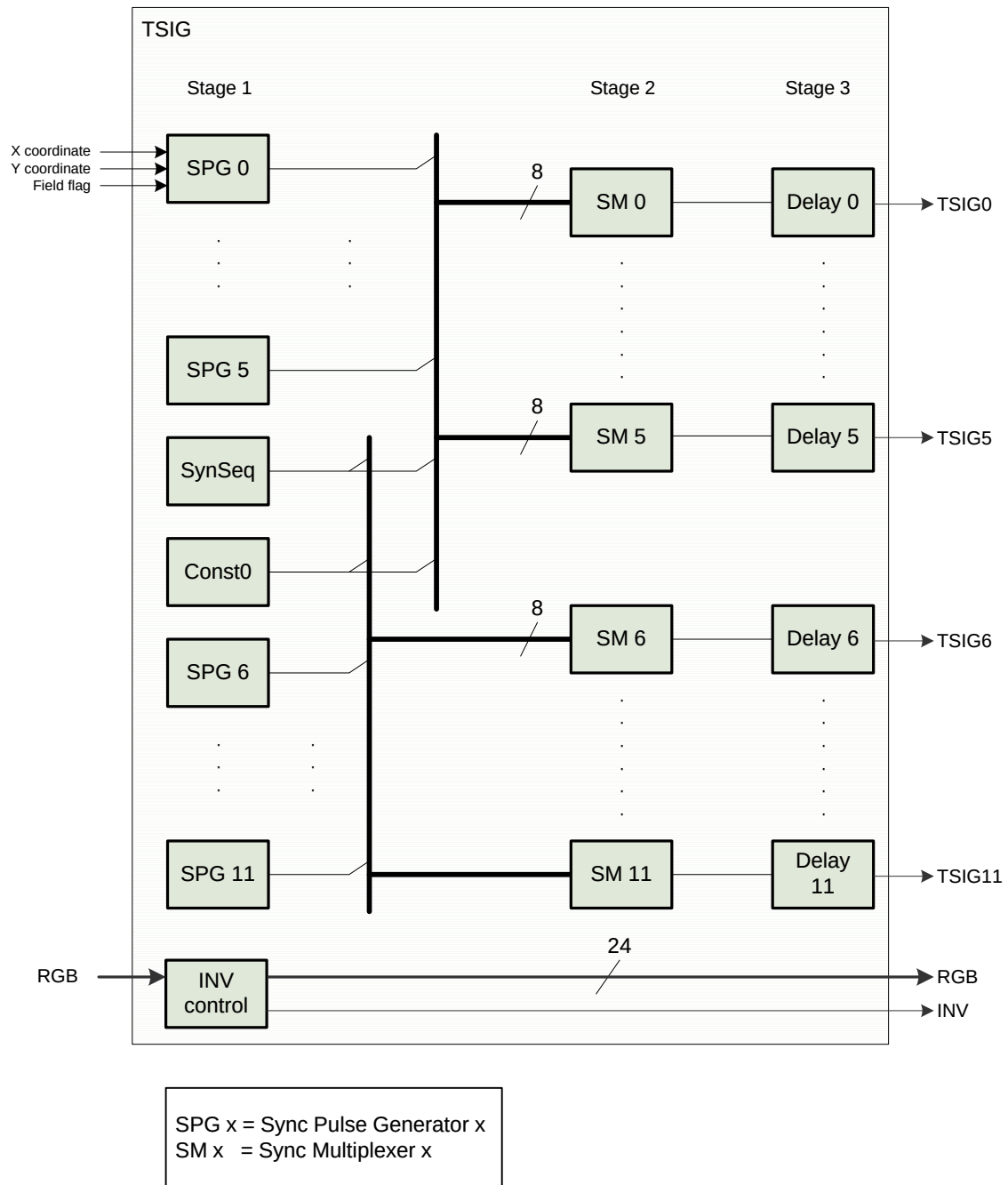
Figure 10-1 Timing Controller module
