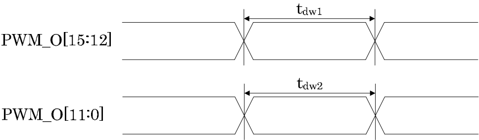
Figure 32-7 PWM Output timing
