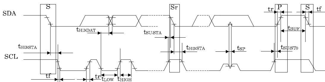
Figure 32-8 I 2 C access timing
