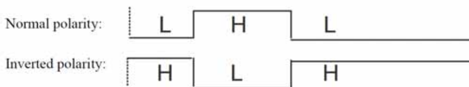
Figure 29-3 One-shot waveform (Rectangular wave)
