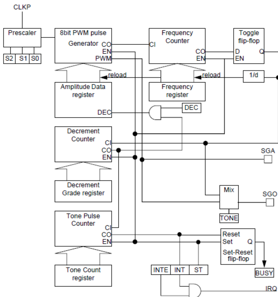
Figure 24-2 Detailed Structure of the sound generator
