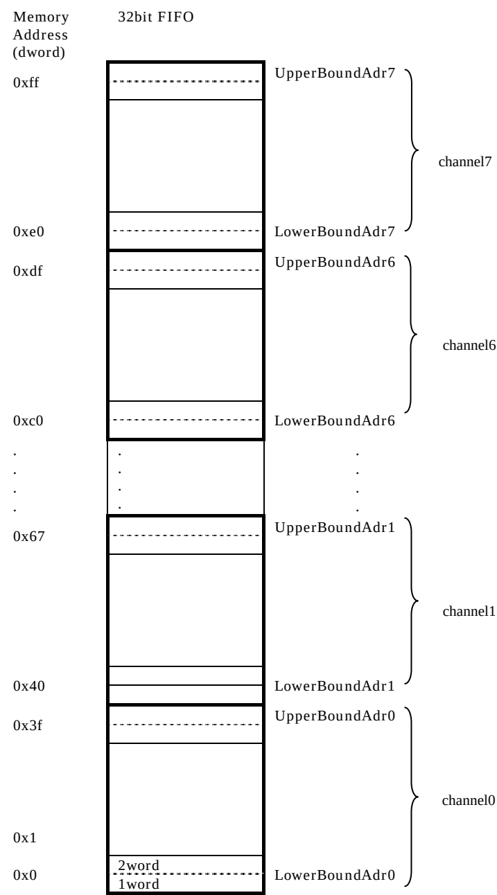
Figure 22-2 FIFO Address setting example
