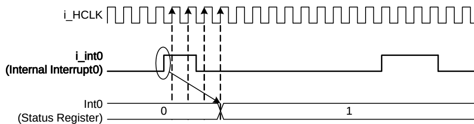
Figure 21-2 Timing diagram of interrupt detection
