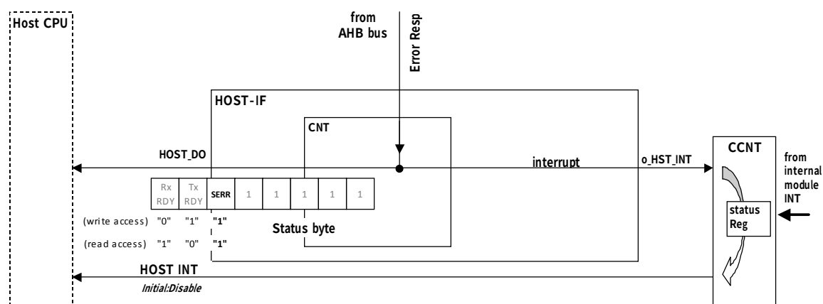
Figure 4-6 Interrupt
