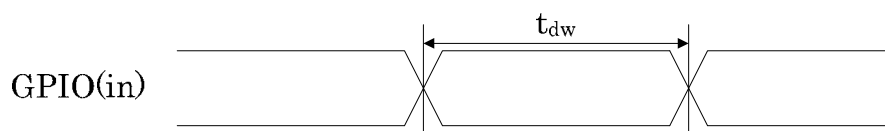
Figure 32-5 GPIO Timings
