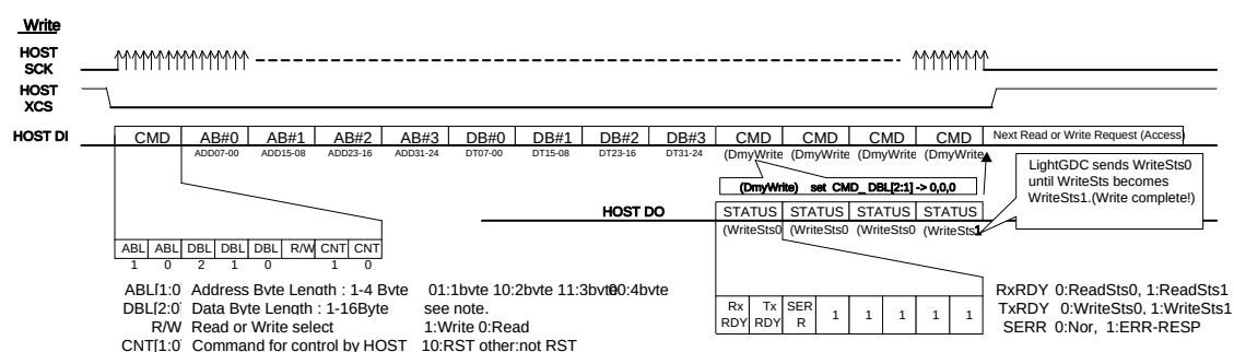
Figure 4-2 Write access
