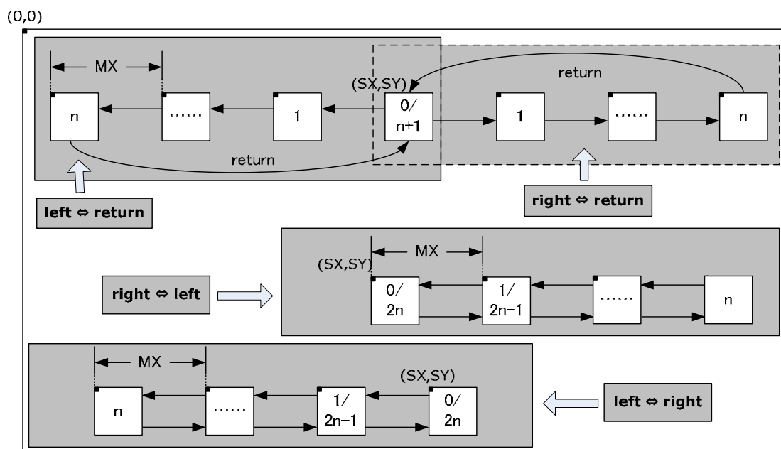
Figure 8-16 Specific movement in X direction
