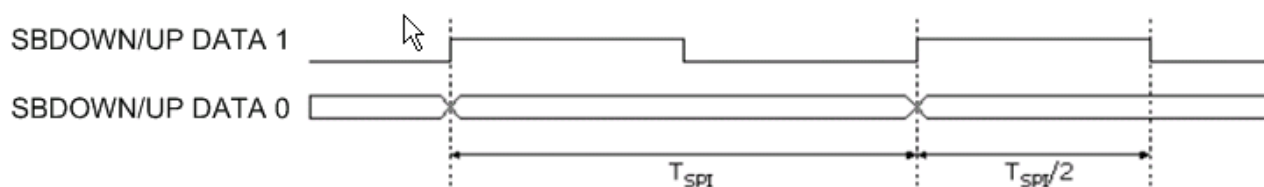
Figure 6-4 SPI-mode
