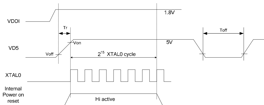
Figure 32-2 Power ON Sequence
