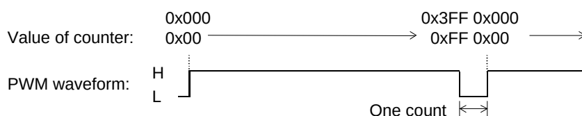
Figure 23-6 Examples of PWM1&2 Waveform Output
