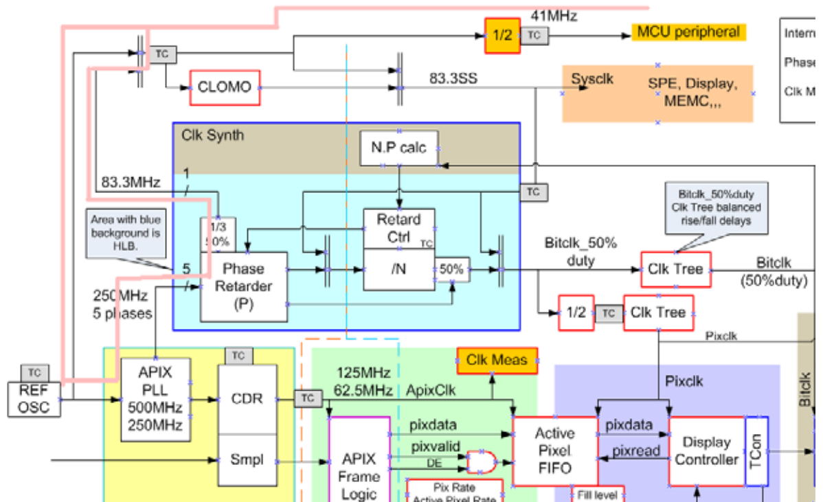
Figure 19-1 Block diagram of CRG module
