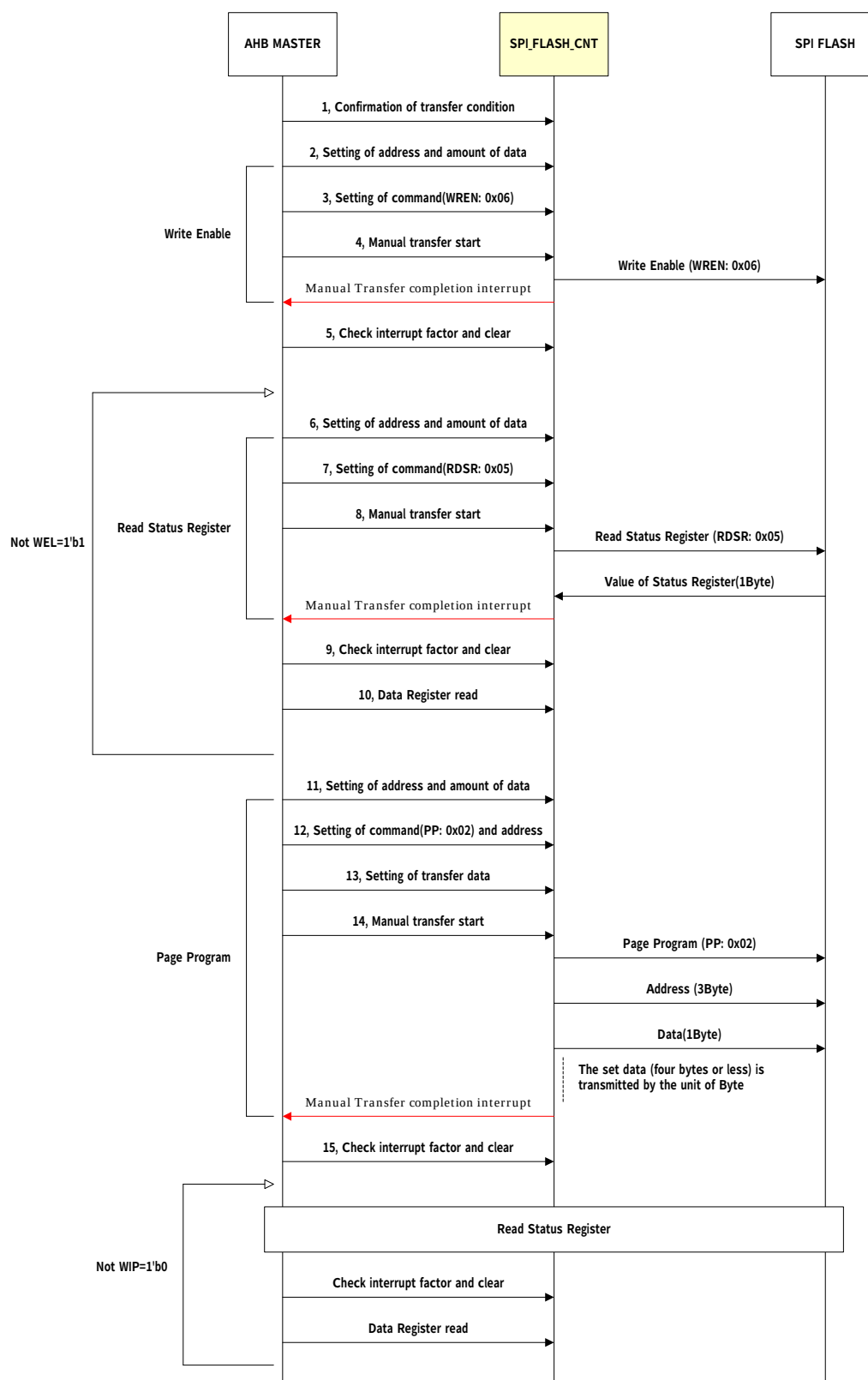
Figure 14-3 Manual Write flow
