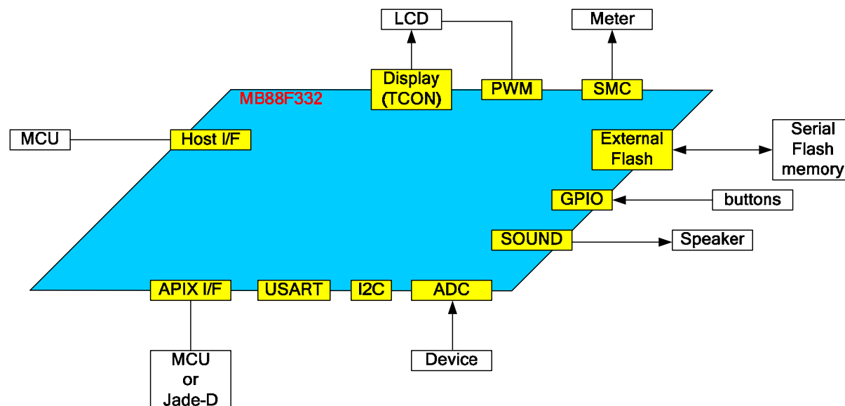
Figure 2-1 MB88F332 system configuration example
