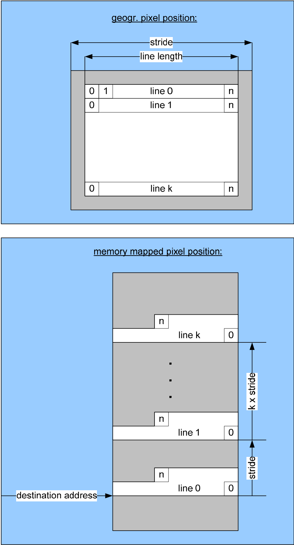
Figure 17-5 Memory Stride
