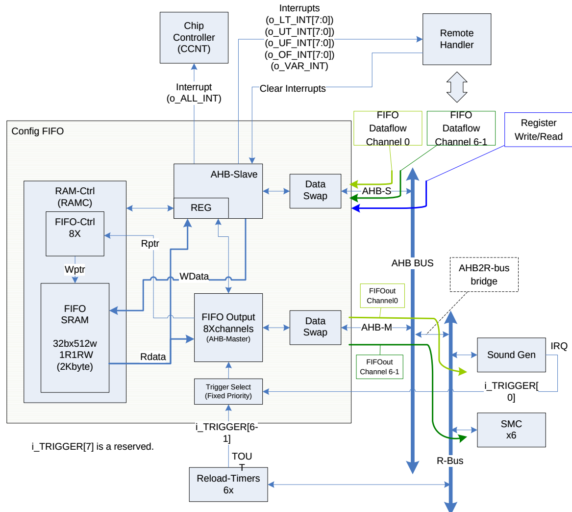
Figure 22-1 Configuration FIFO block
