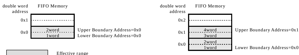
Figure 22-3 FIFO Address setting example.
