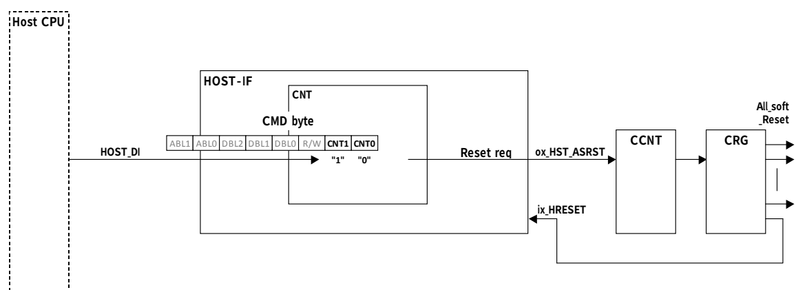
Figure 4-7 Reset request
