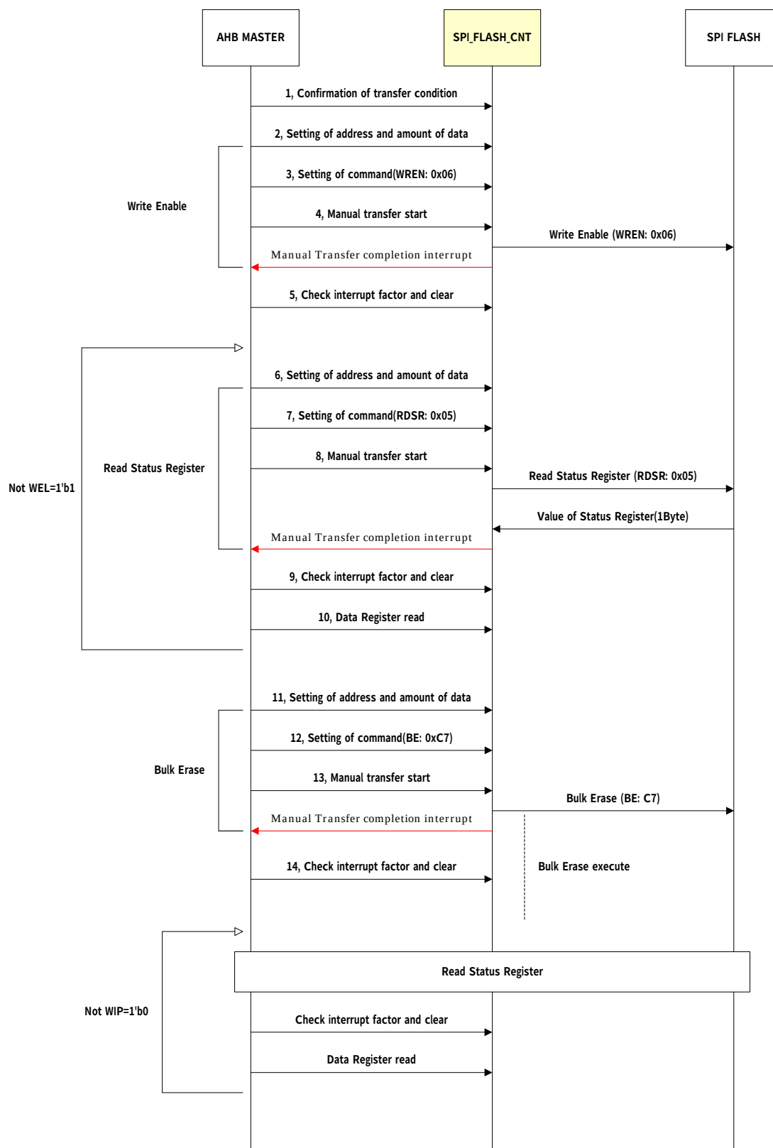
Figure 14-6 Manual Bulk Erase flow
