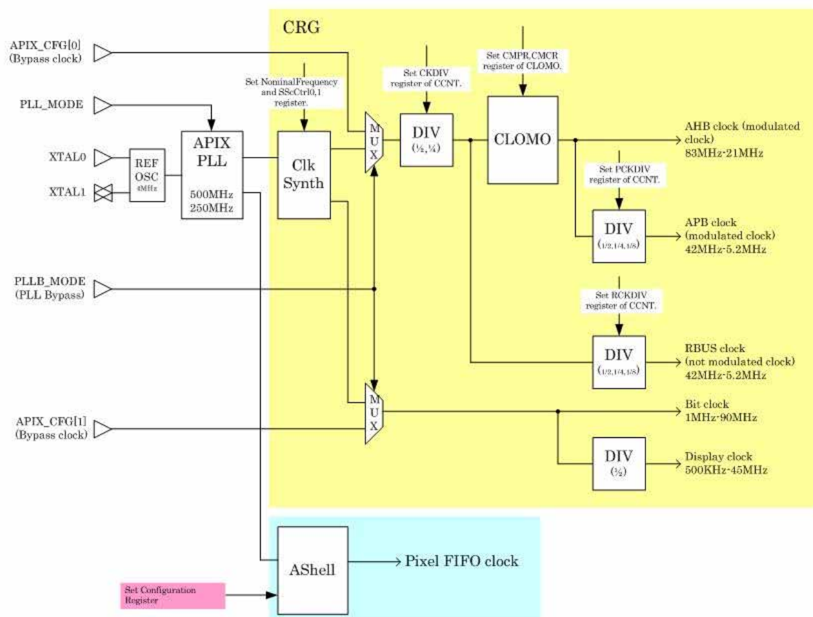
Figure 1-2 MB88F332 Indigo Clock Generation
