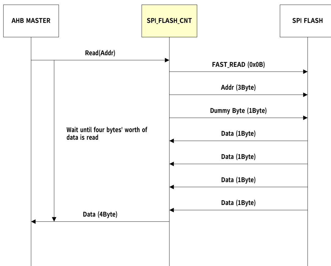
Figure 14-2 Slave Read Mode flow
