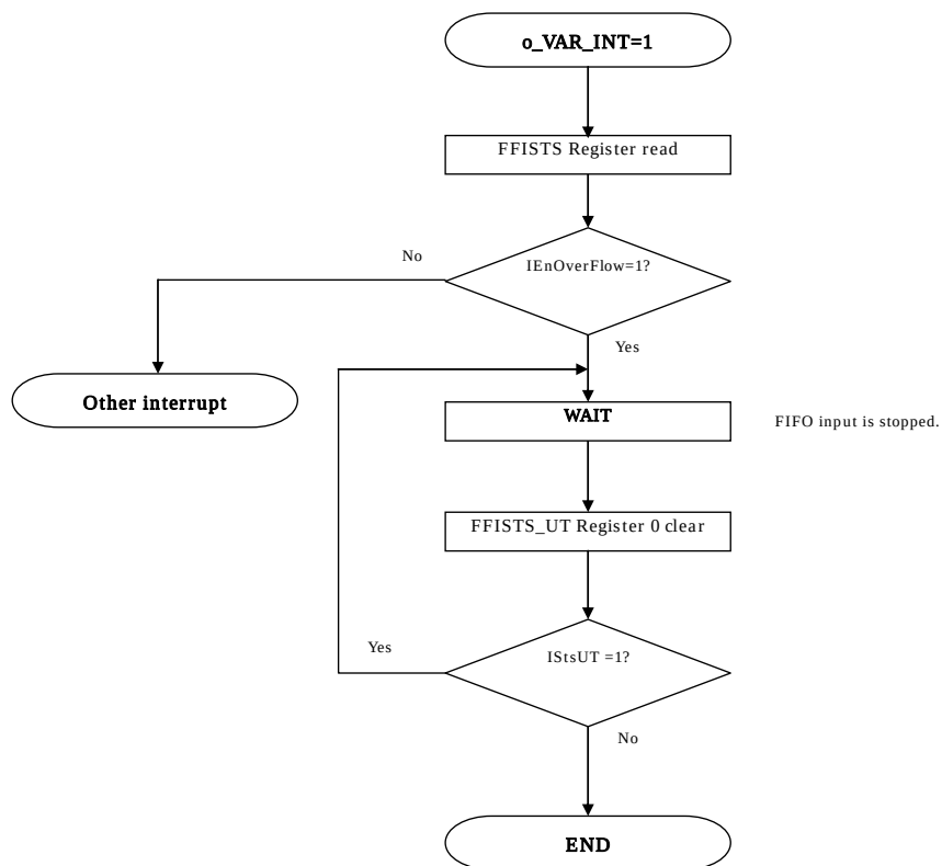
Figure 22-14 FIFO Full Flow
