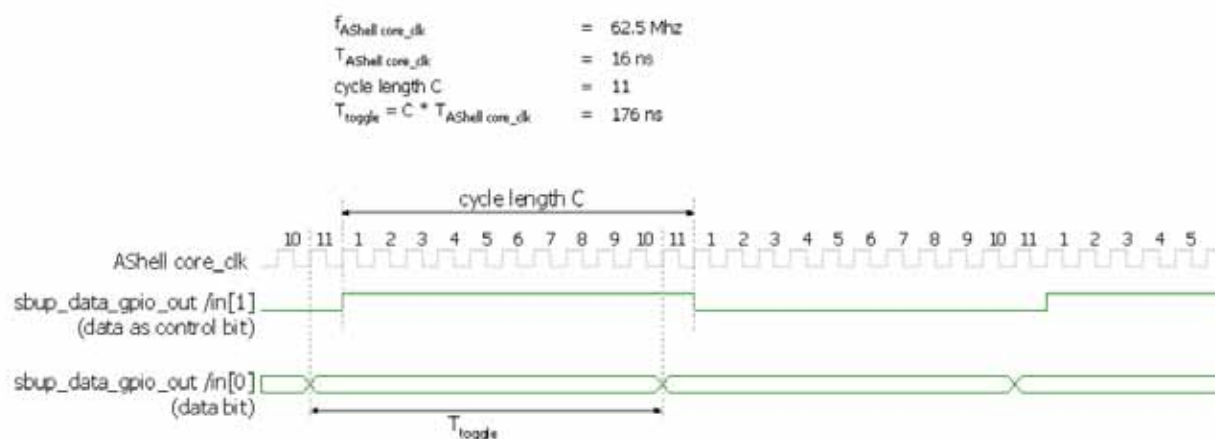
Figure 6-5 timing diagram of toggle mode
