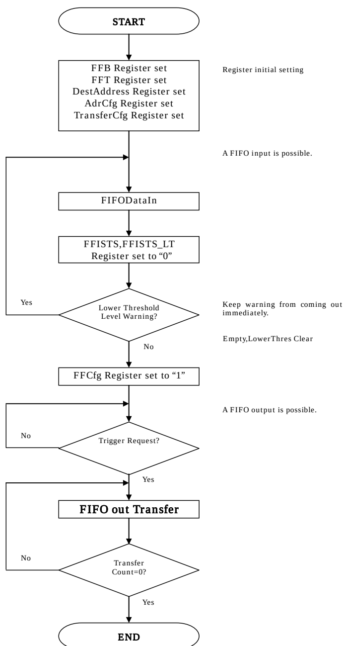
Figure 22-9 Register Initial Setting Flow
