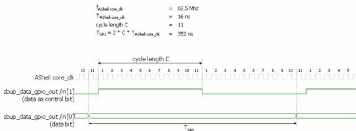
Figure 6-6, timing diagram of SPI mode
