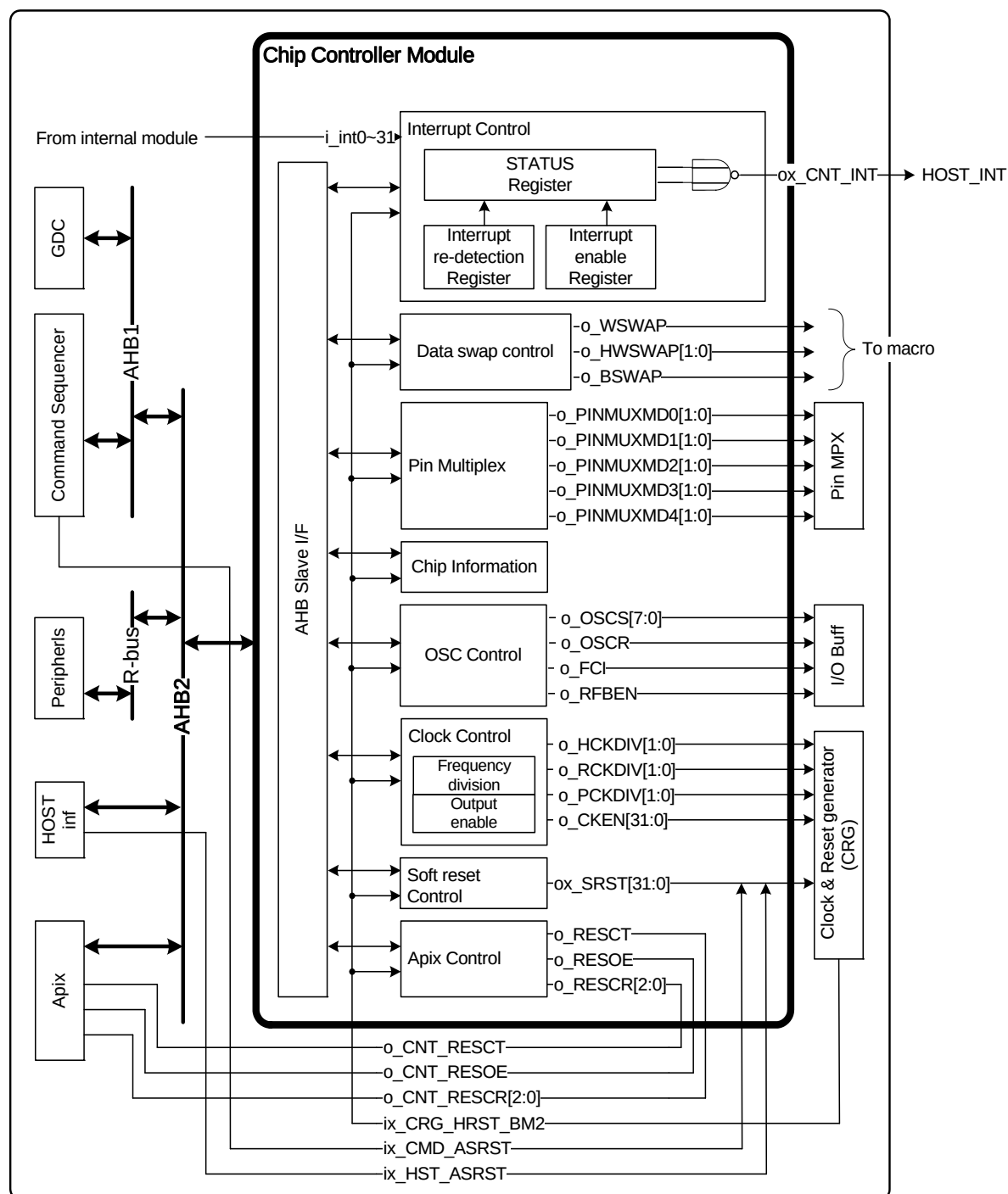
Figure 21-1 Block diagram of CCNT
