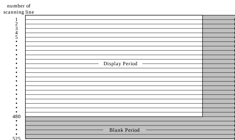
Figure 9-11 Progressive scan
