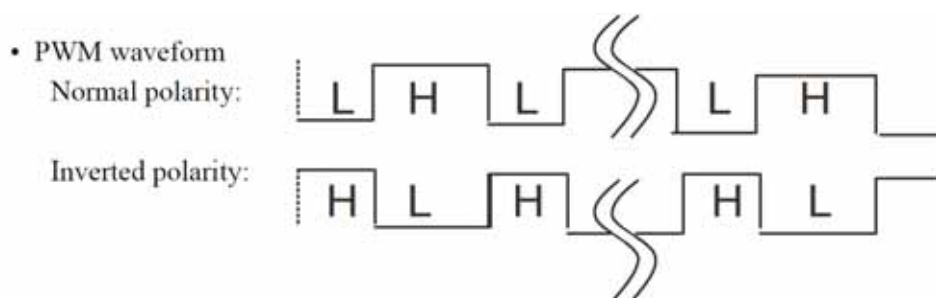
Figure 29-2 Output waveforms
