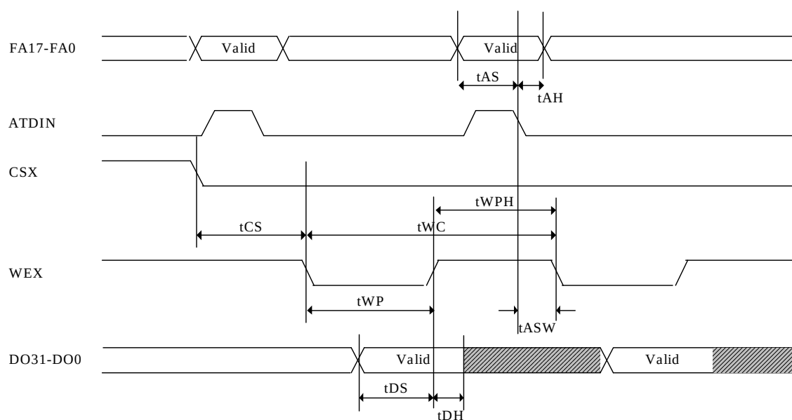
Figure 15.6-2 Synchronous Write
