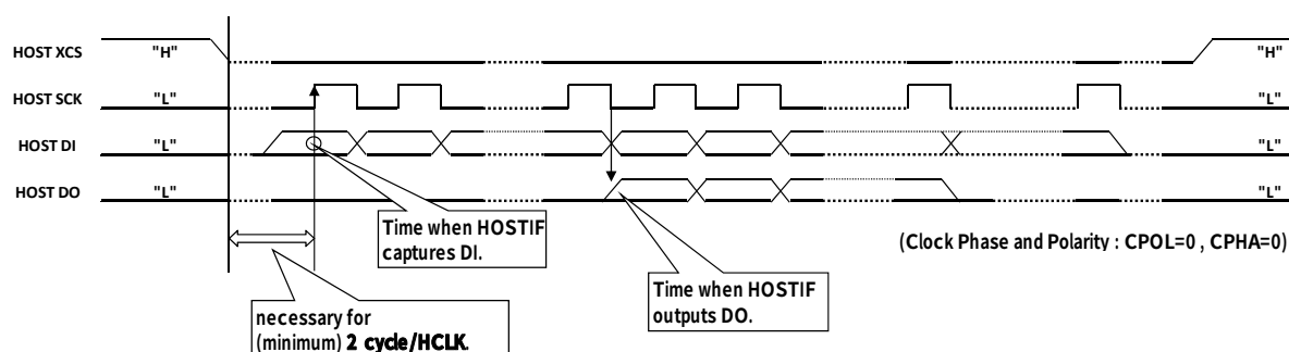
Figure 4-9 Host Interface (clock timing and phase)
