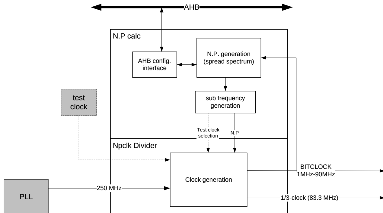
Figure 19-2 Block diagram of ClkSynth module
