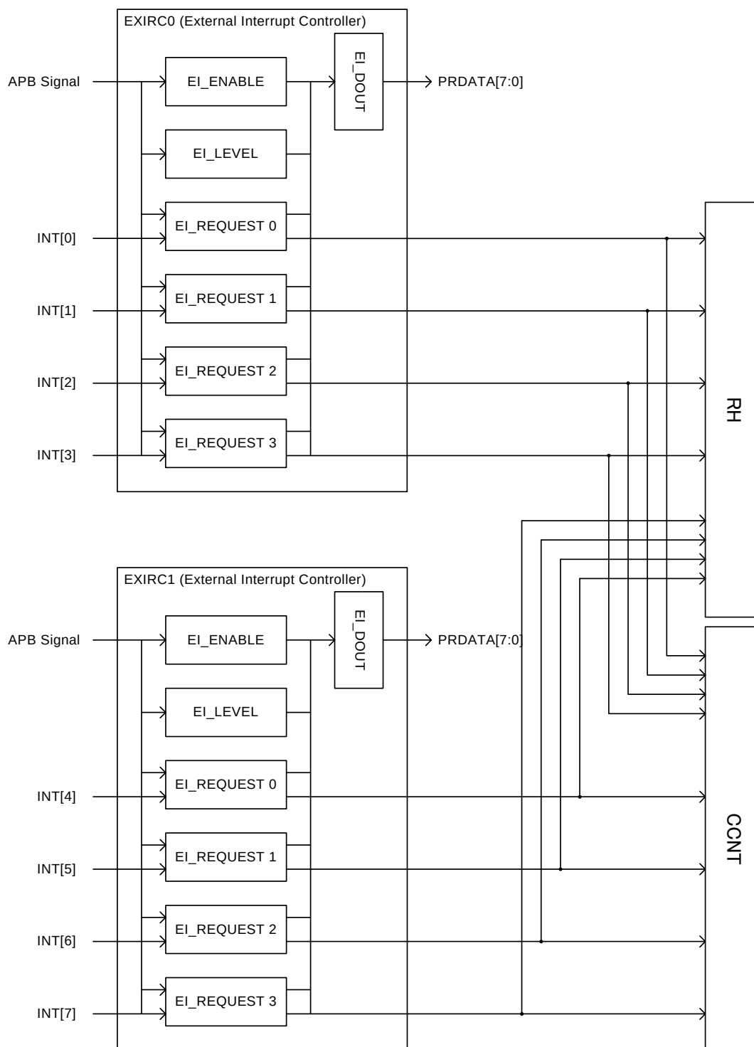
Figure 28-1 Block Diagram of External Interrupt Controller
