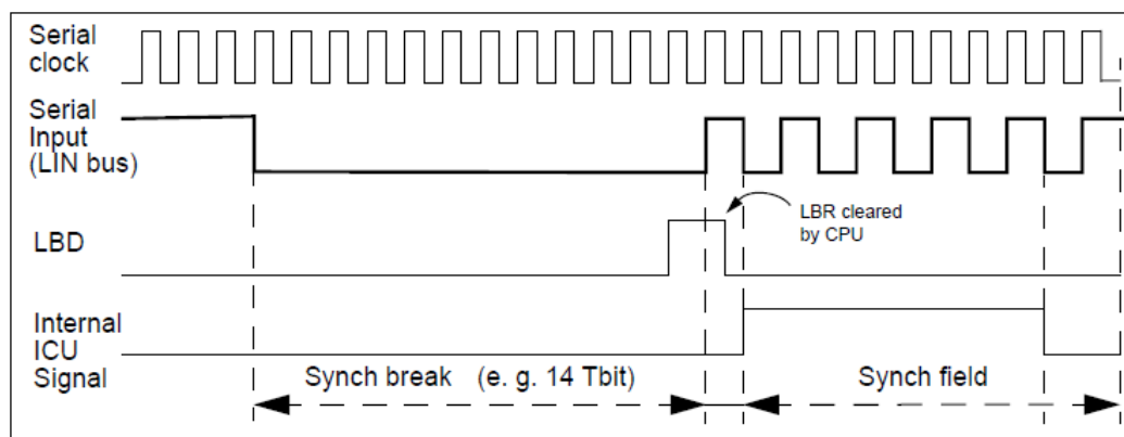
Figure 26-14 USART behavior as slave in LIN mode
