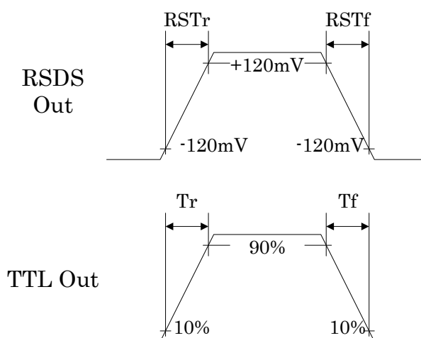
Figure 32-10 Rise Fall Times
