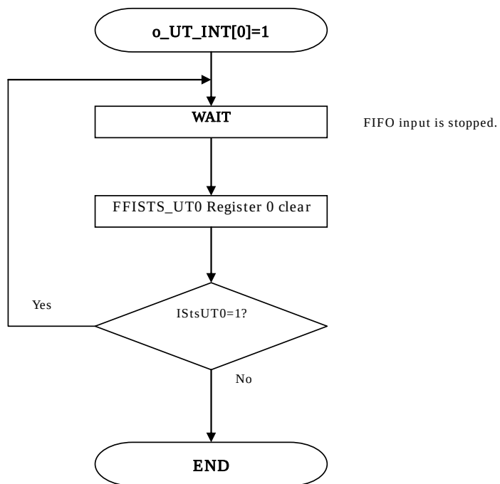
Figure 22-13 FIFO Upper Threshold Warning Flow
