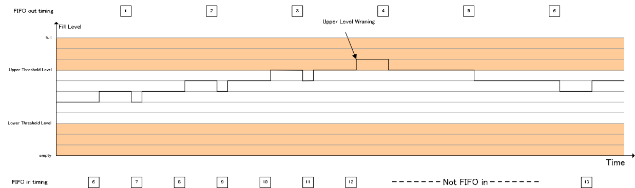
Figure 22-7 FIFO Flow (Upper Threshold Warning)
