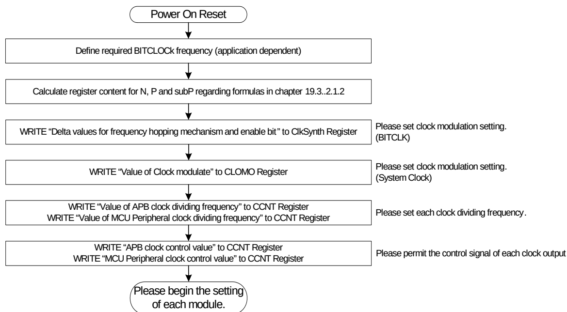
Figure 19-4 Clock setting flow
