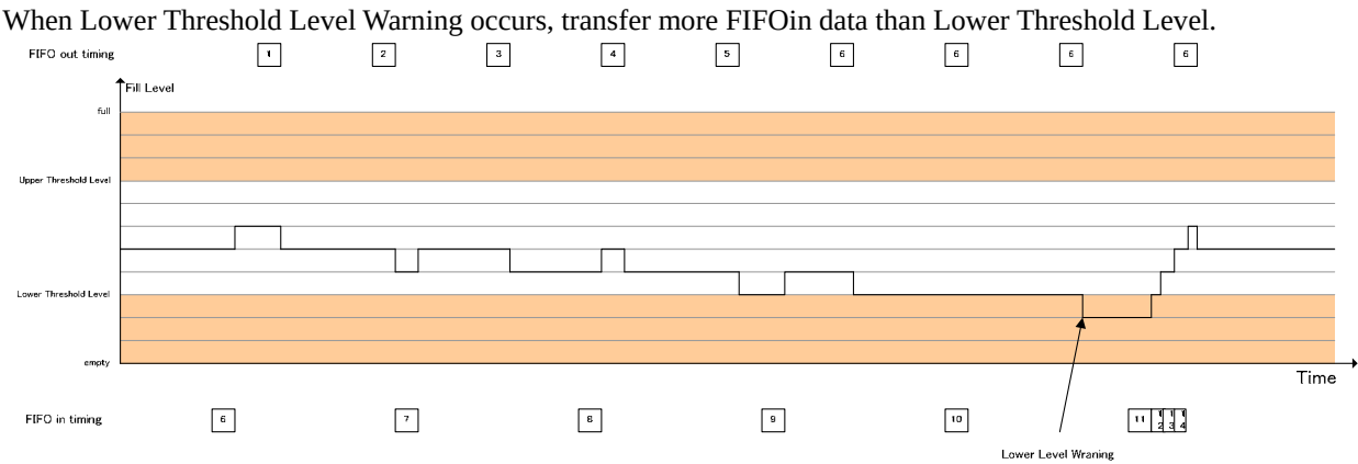
Figure 22-8 FIFO Flow (Lower Threshold Warning)
