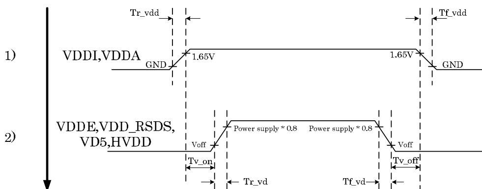
Figure 32-1 Recommended Power ON/OFF Sequence
