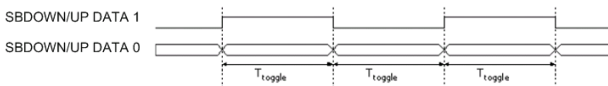
Figure 6-3 Toggle Mode
