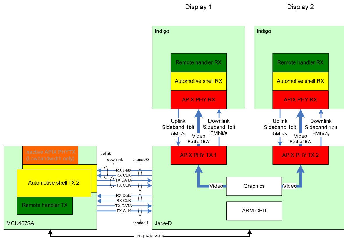
Figure 5-3, High-Quality Dual Display application (variant 1) 2
