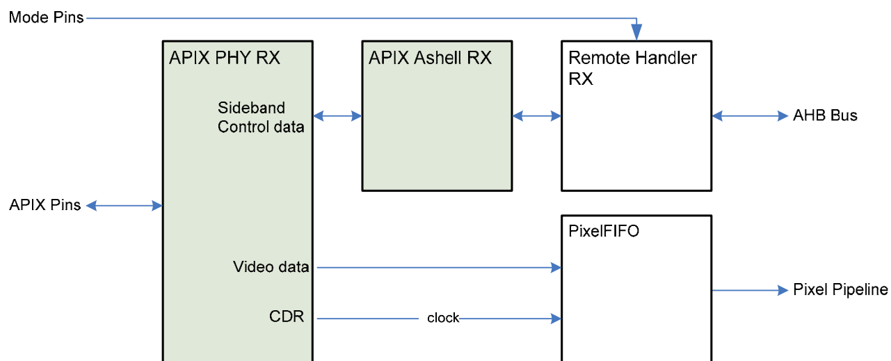
Figure 5-1 Block diagram of APIX® PHY RX and APIX Ashell® RX in the System
