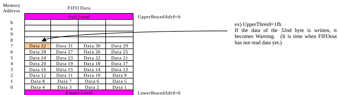
Figure 22-4 Upper threshold warning
