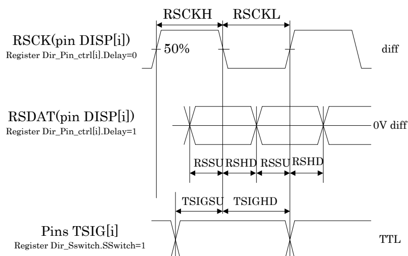
Figure 32-11 RSDS operation Output Timing
