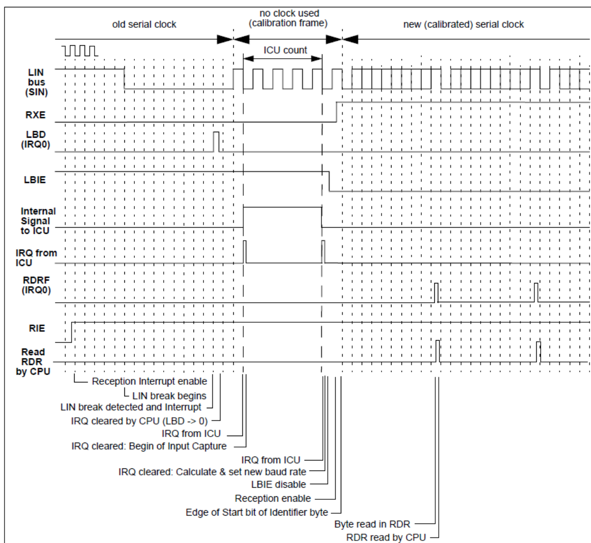
Figure 26-15 LIN bus timing and USART signals
