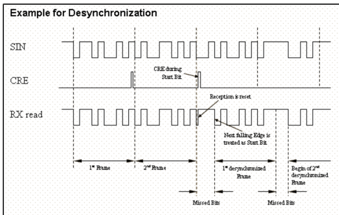
Figure 26-27 Data Stream Synchronization
