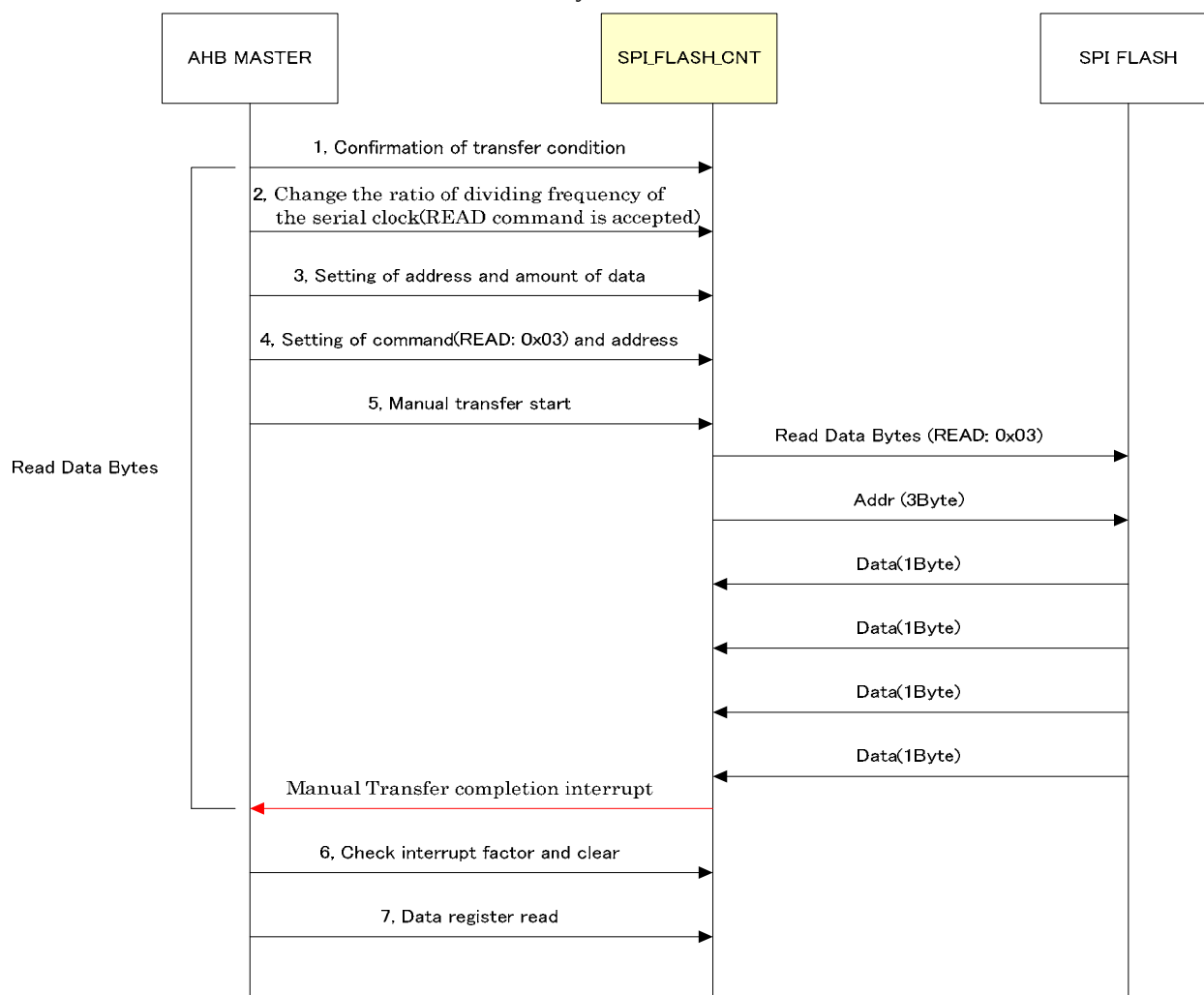
Figure 14-4 Manual Read flow
