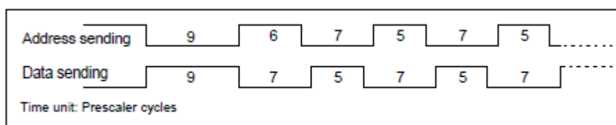
Figure 25-18 SCL Waveforms
