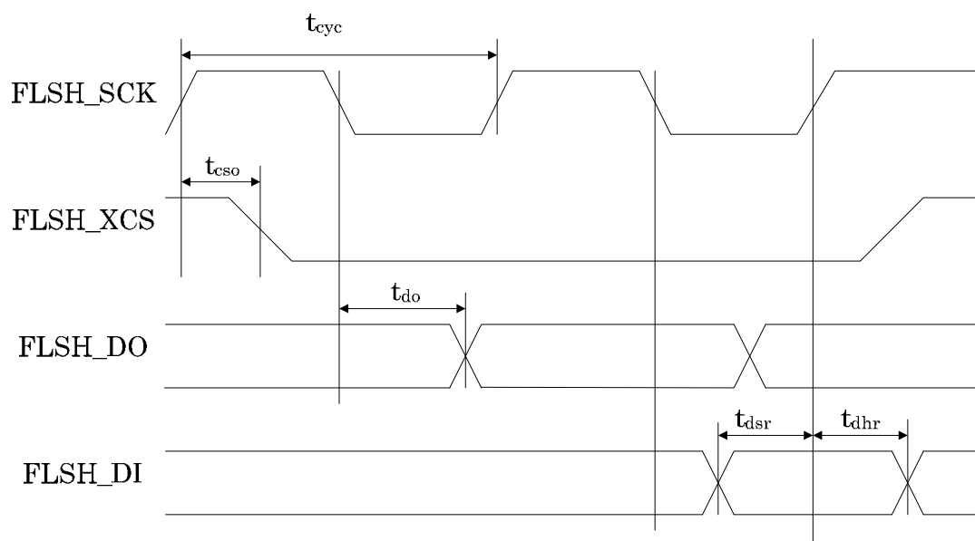
Figure 32-3 External Serial Flash I/F Timings
