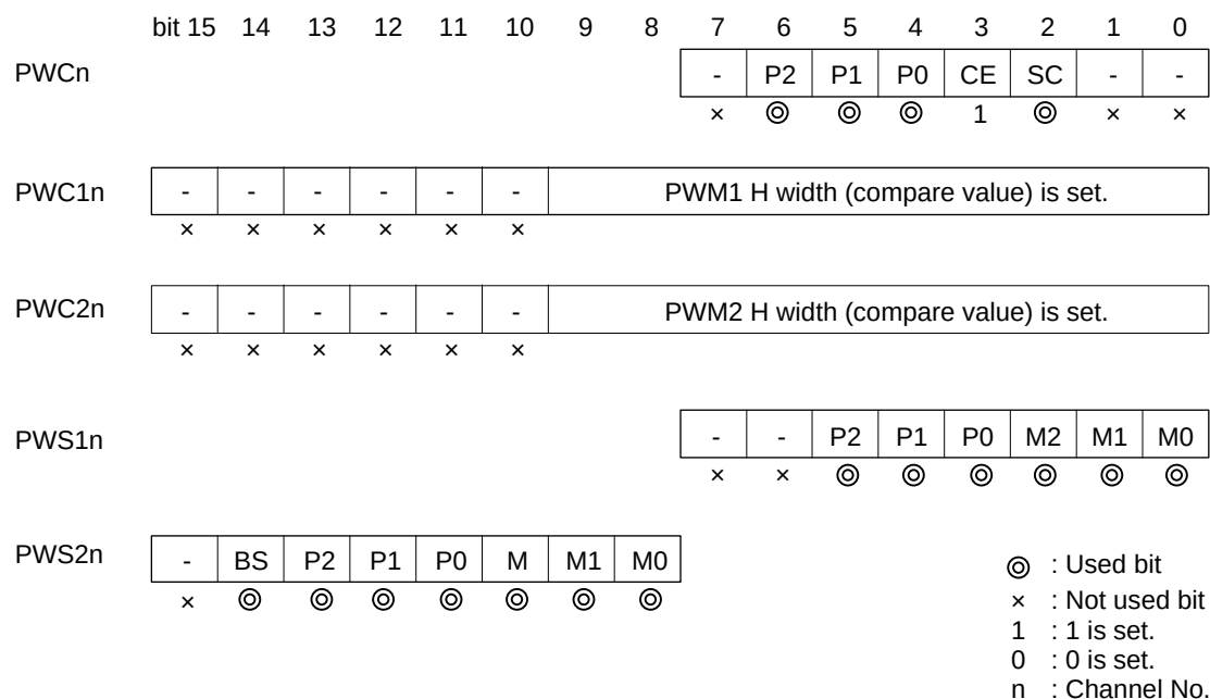
Figure 23-5 Setting of Stepper motor controller
