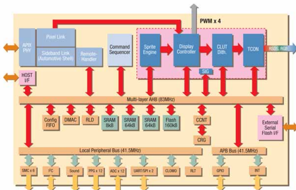
Figure 1-1 Block diagram of MB88F332
