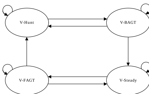
Figure 9.3-5 External Synchronization State Machine
