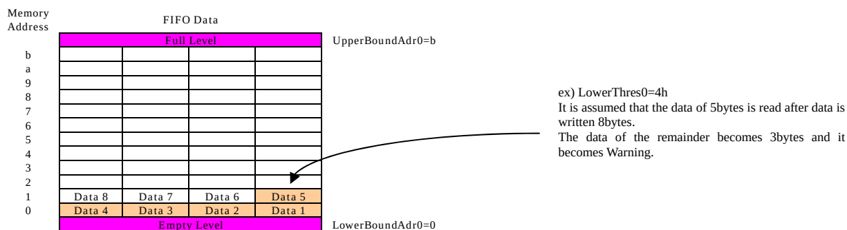
Figure 22-5 Lower threshold warning
