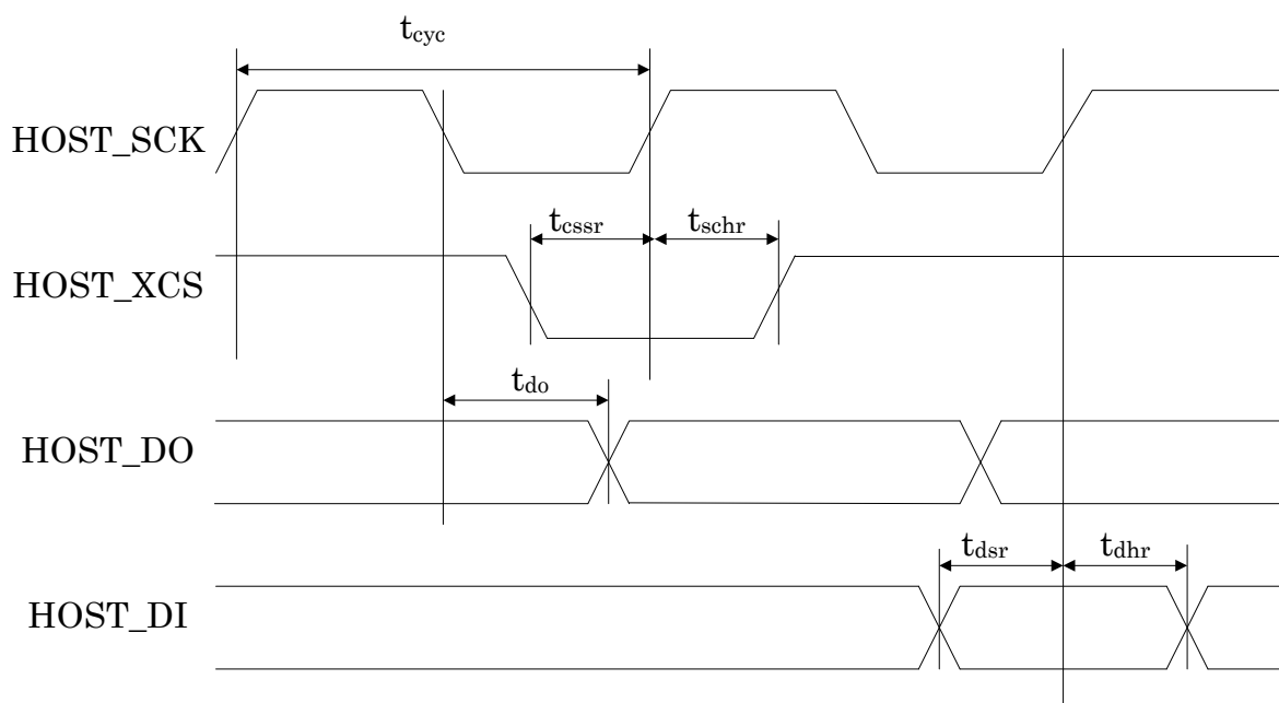
Figure 32-4 Host I/F Timings
