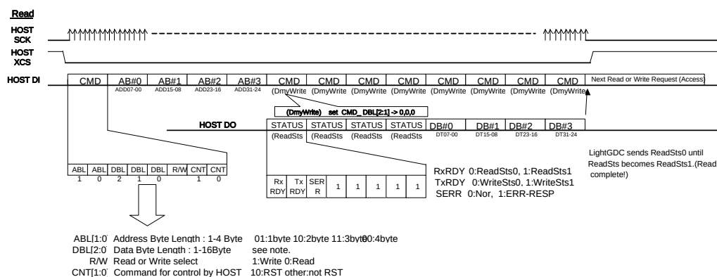
Figure 4-4 Read access
