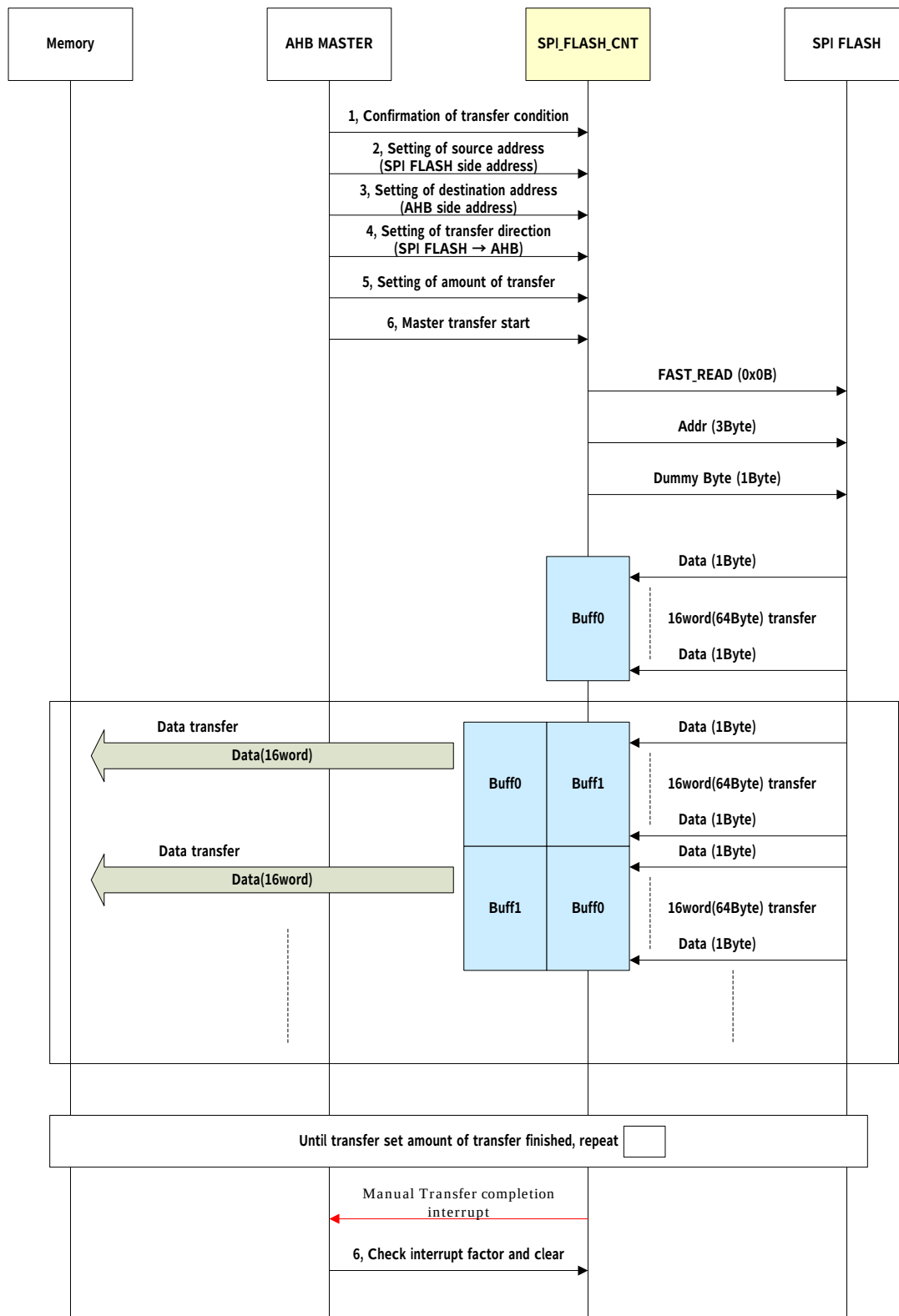
Figure 14-8 Master Read flow
