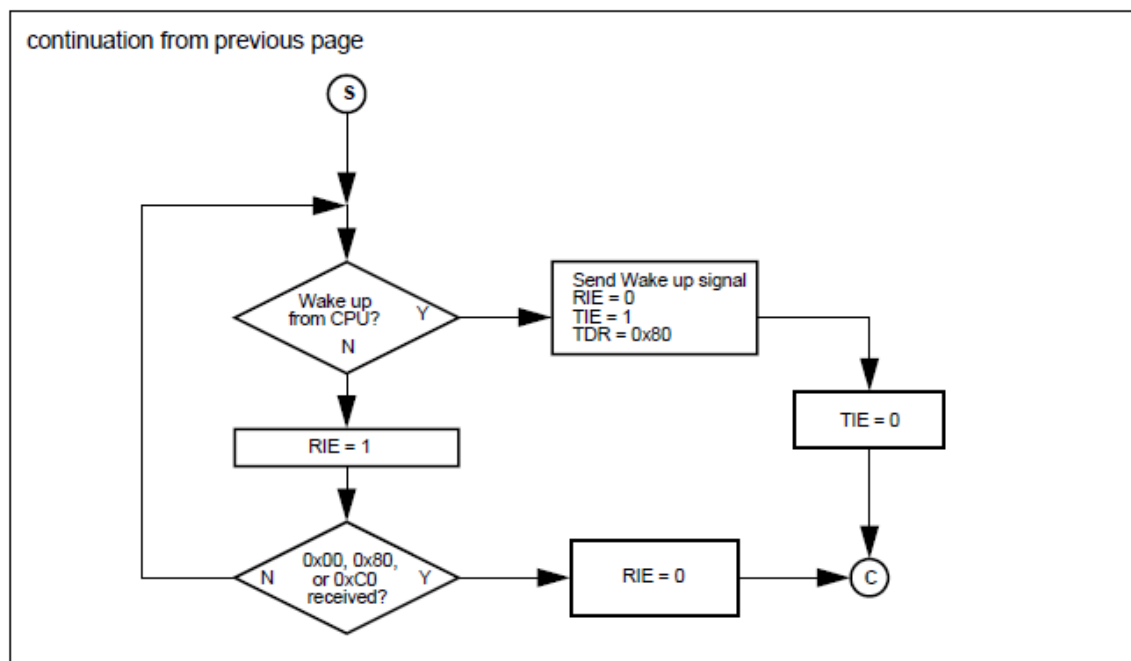
Figure 26-25 USART LIN slave flow chart (part 2)
