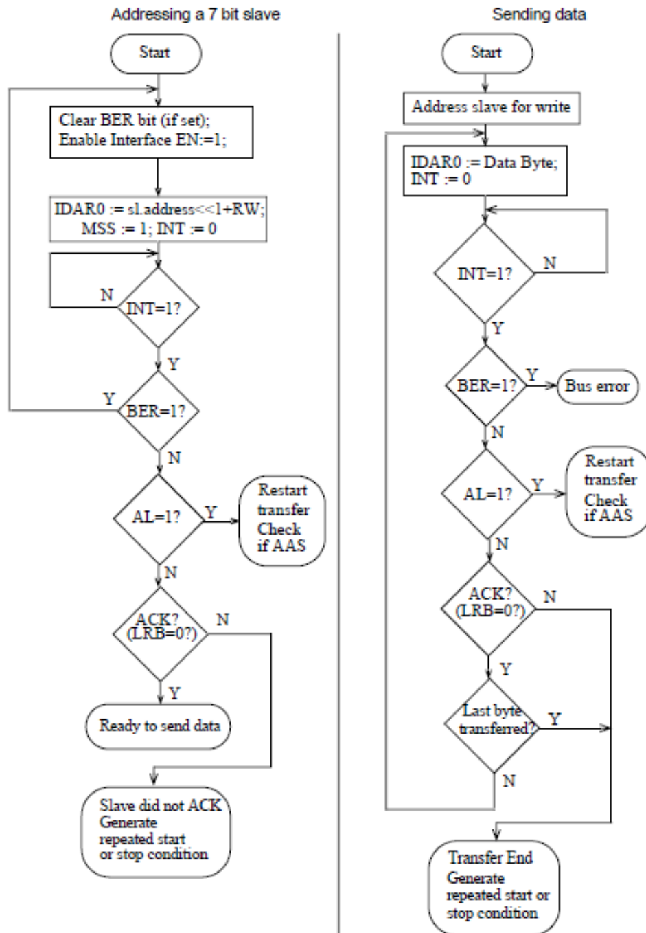
Figure 25-19 Example of Slave Addressing and Sending Data
