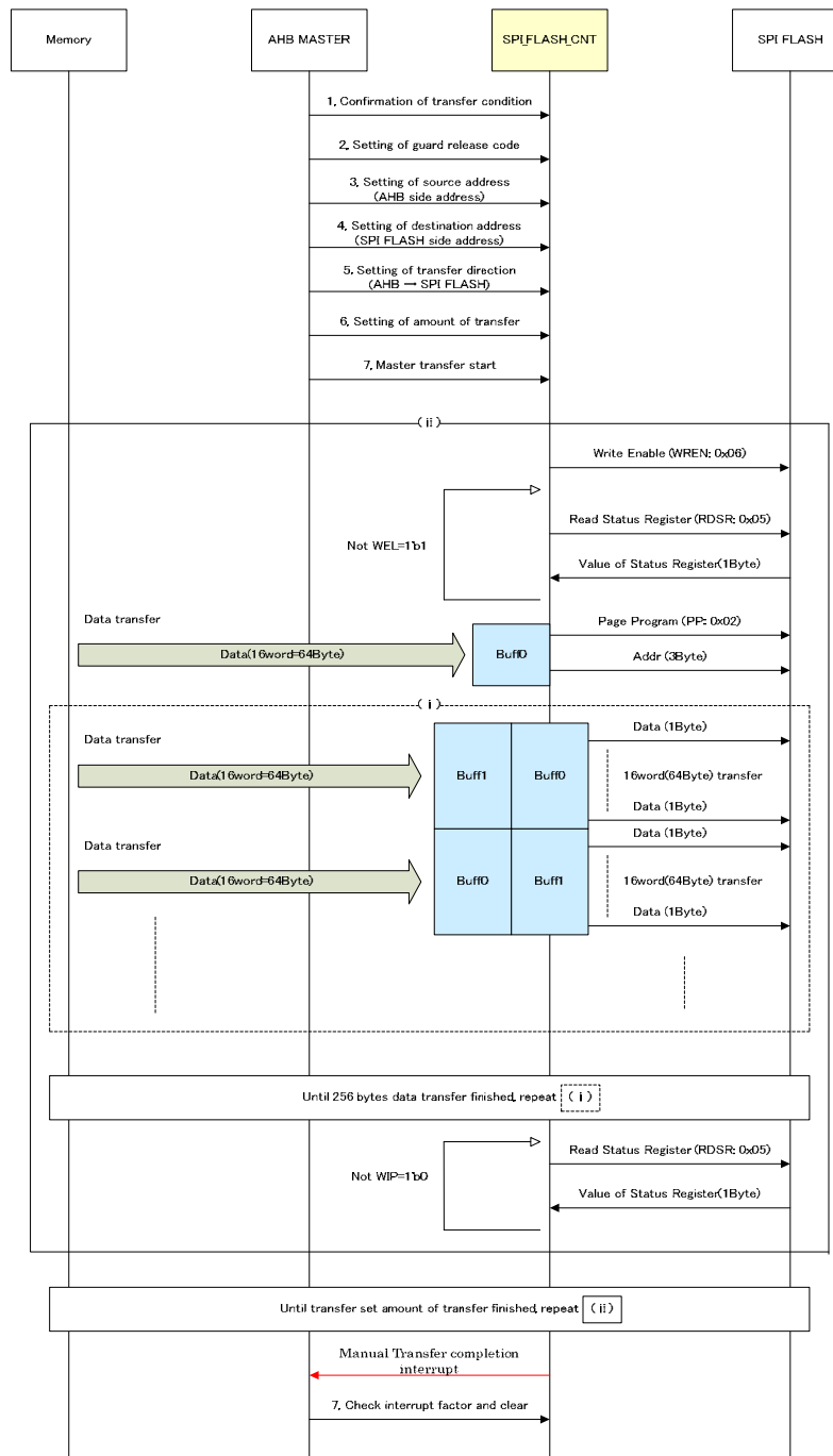
Figure 14-7 Master Write flow
