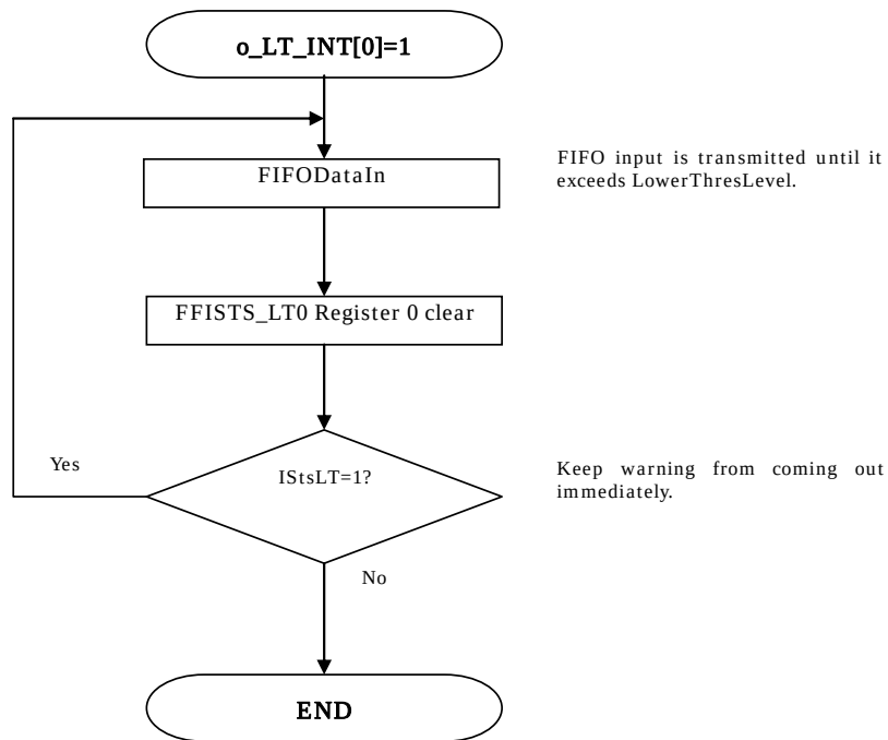
Figure 22-11 FIFO Lower Threshold Warning Flow
