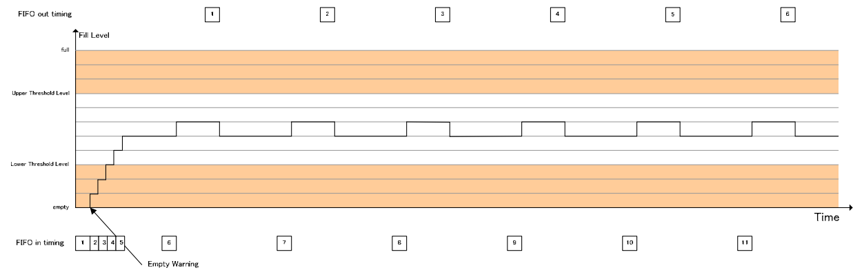
Figure 22-6 FIFO Flow (Empty Warning)
