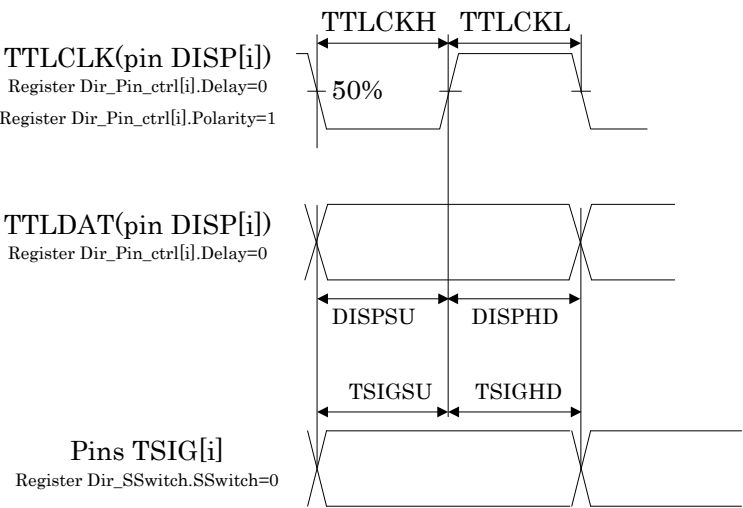
Figure 32-13 TTL operation output timing (not bypass mode) (2)
