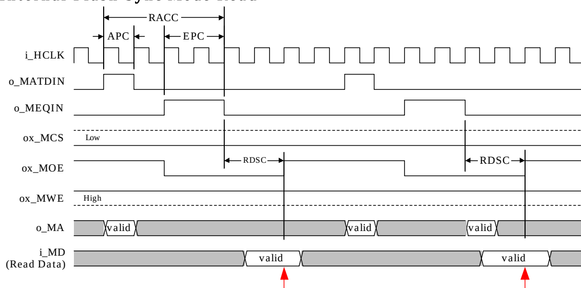
Figure 15.3-3 Flash Read Access
