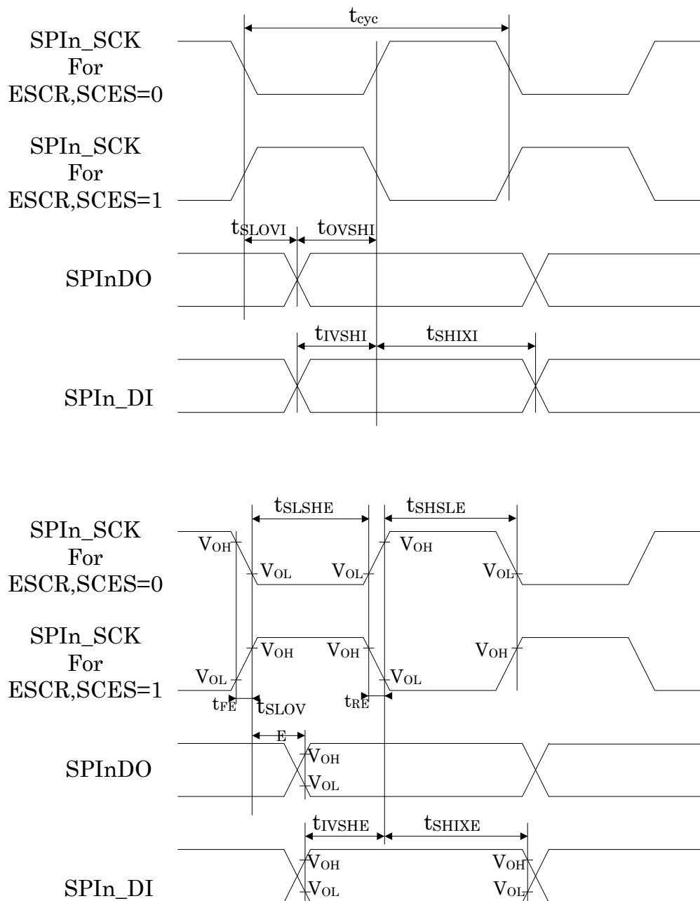
Figure 32-9 SPI Timings
