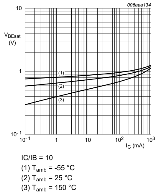
Fig. 5. BC817-16W: Base-emitter saturation voltage as a function of collector current; typical values
