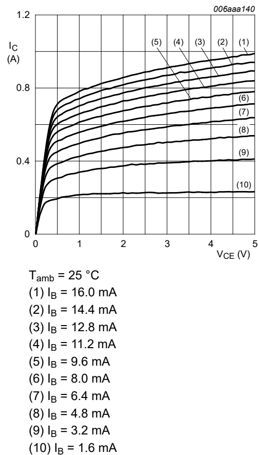
Fig. 7. BC817-16W: Collector current as a function of collector-emitter voltage; typical values
