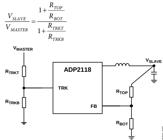
Figure 42. Voltage Tracking
