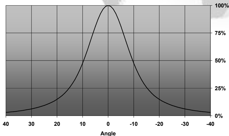
Relative Intensity of LISA-O1-SS
