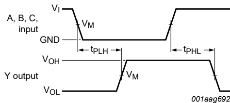
Fig. 5. The input (A, B, C) to output (Y) propagation delays
