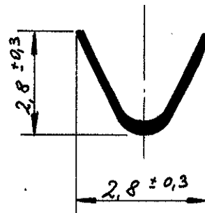
ISOL. PRESSHÜLSE
