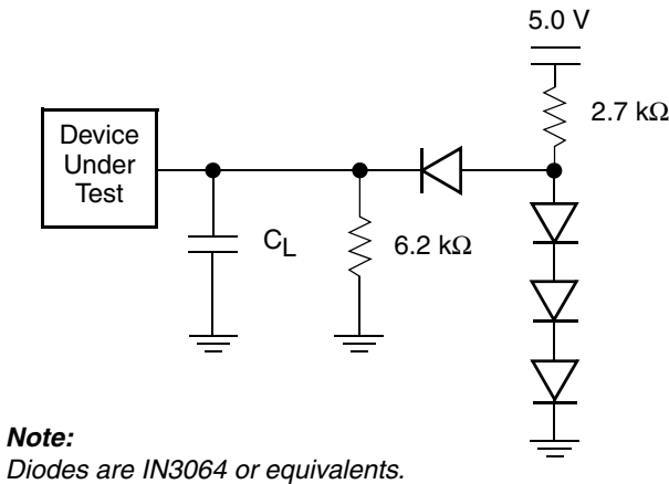
Figure 8. Test Setup
