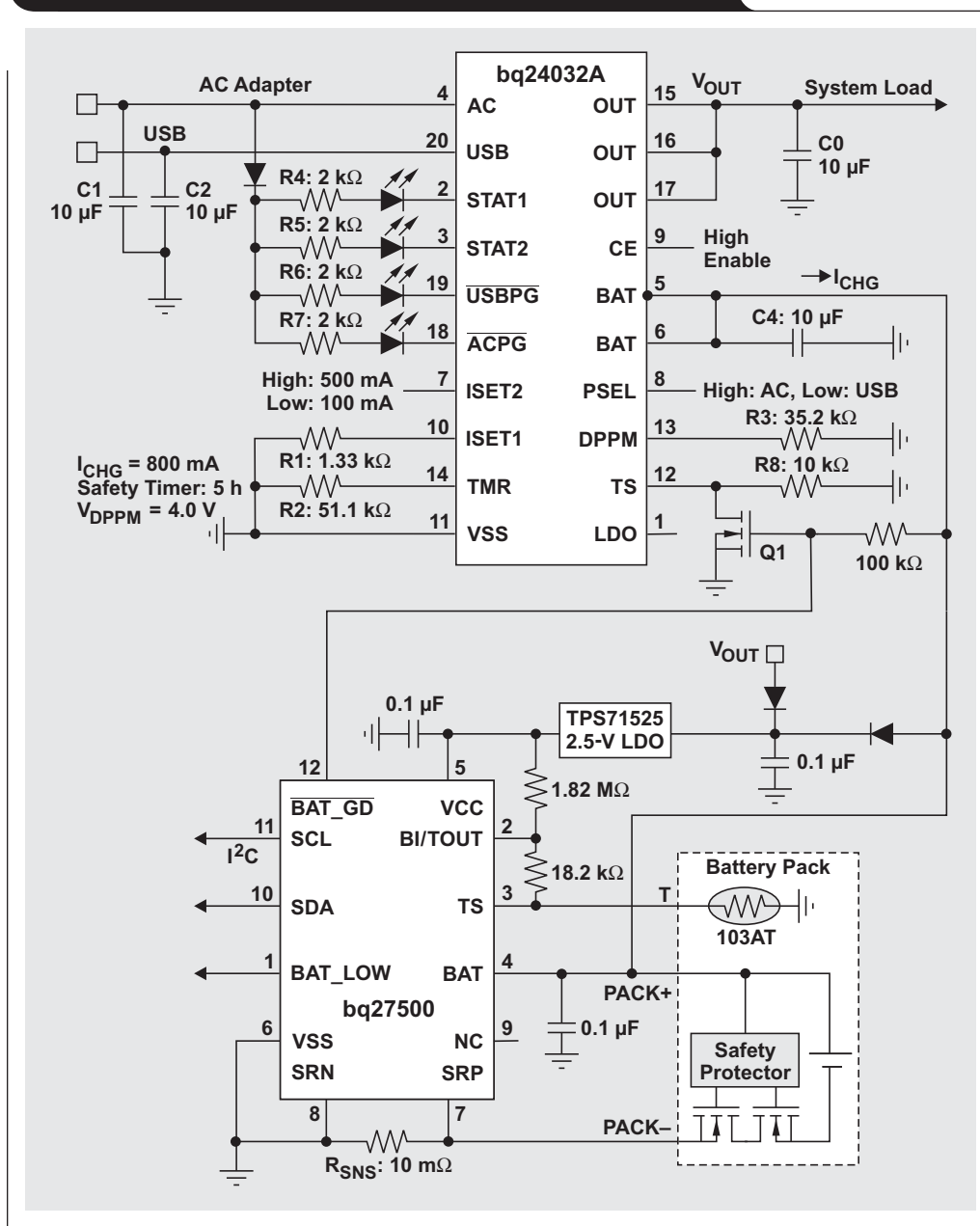
Figure 3. Host-side gas-gauge and battery-charging system
