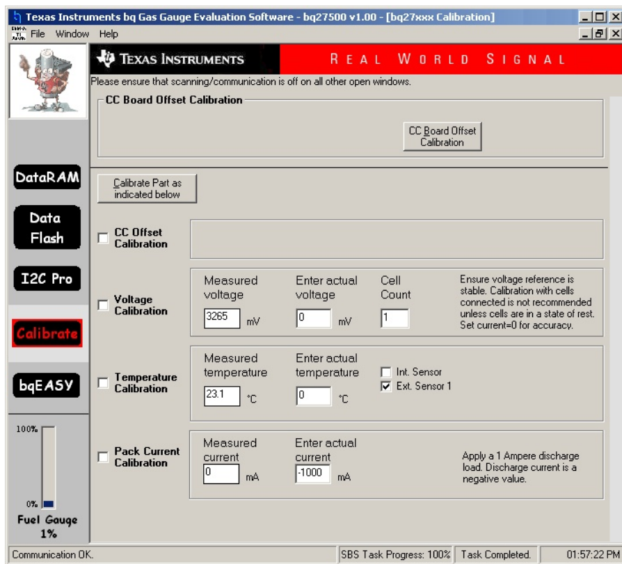
Figure 44. Calibrate Window
