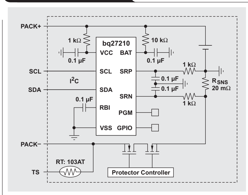
Figure 1. Traditional battery pack
