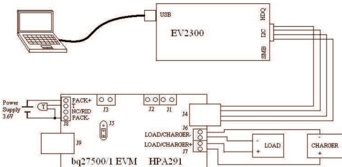
Figure 23. bq27500 Circuit Module Connection to Cell and System Load/Charger
