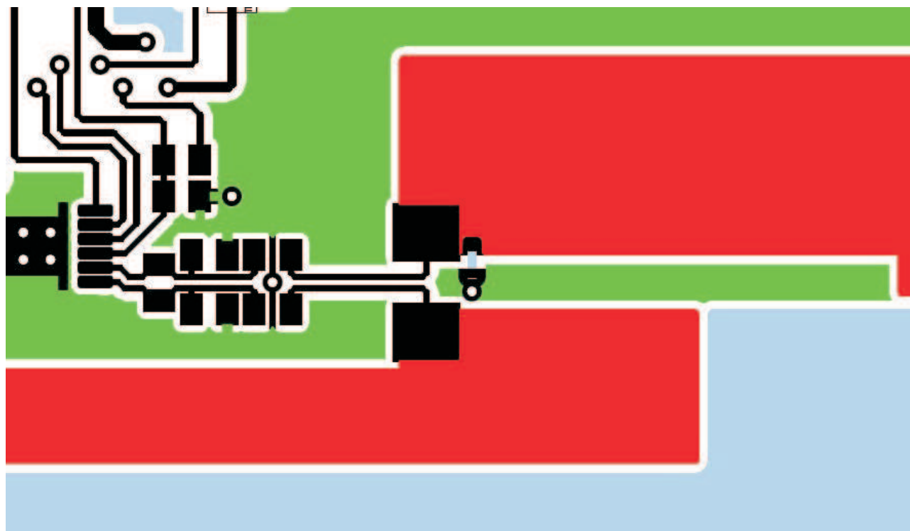
Figure 77. Differential Filter Components With Symmetrical Layout
