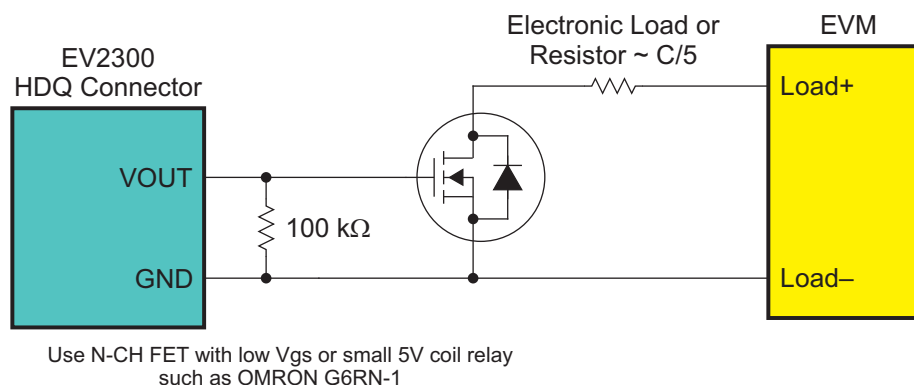
Figure 83. Configuration of Load Circuit
