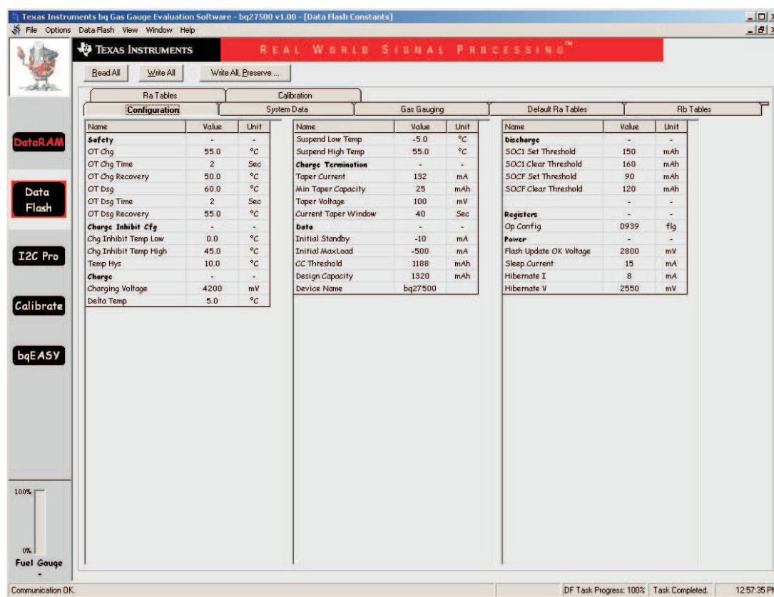
Figure 4. Configuration Screen
