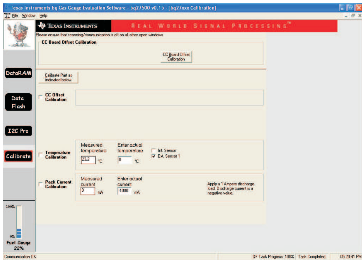
Figure 26. Calibration Screen
