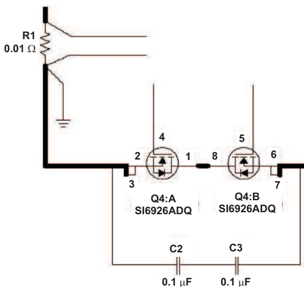
Figure 71. Protection FETs
