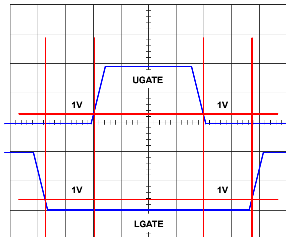
FIGURE 15. GATE DRIVE ADAPTIVE SHOOT-THROUGH PROTECTION
