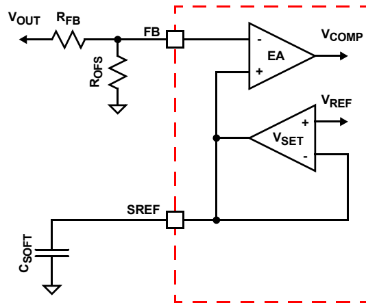
FIGURE 7. ISL95873 VOLTAGE PROGRAMMING CIRCUIT
