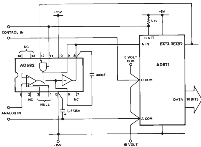
Figure 13. Sample-Hold Interface to the AD571
