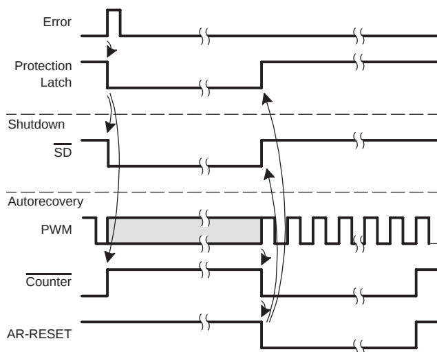
Figure 9. Autorecovery Function
