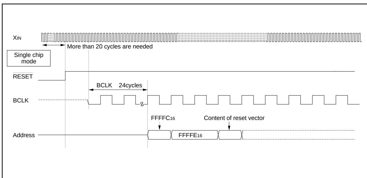
Figure 1.6.2. Reset sequence
