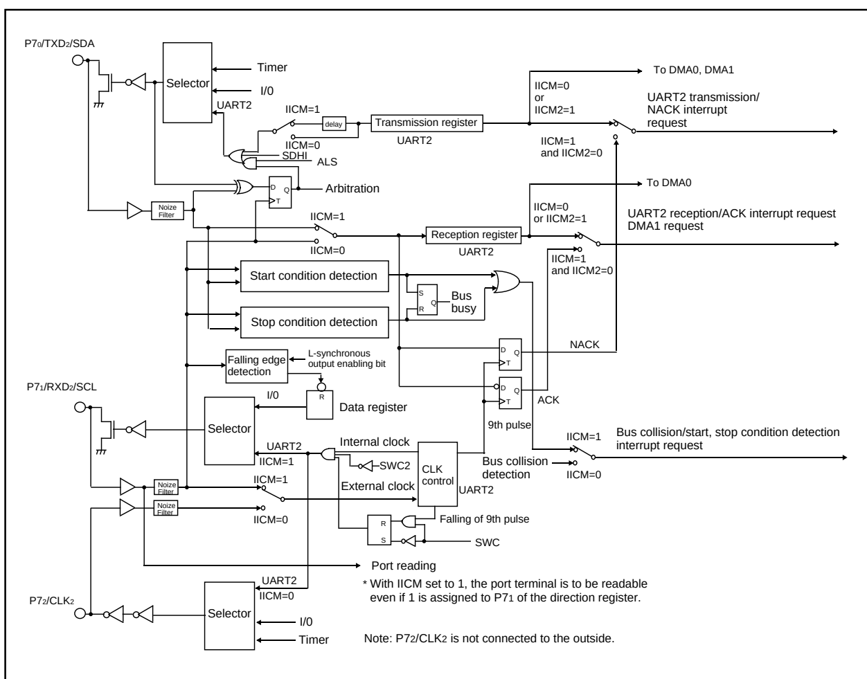
Figure 1.14.30. Functional block diagram for I²C mode
