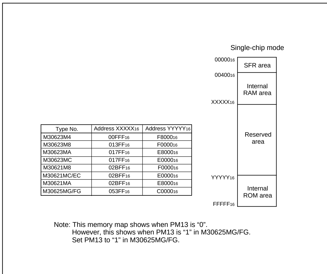
Figure 1.8.2. Memory map
