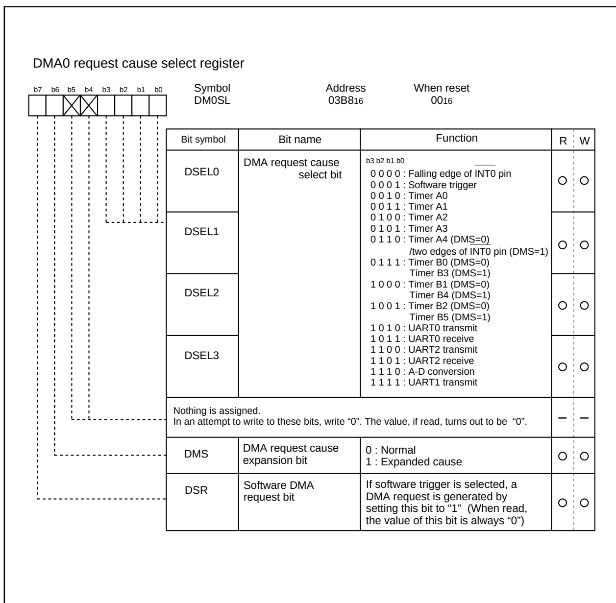
Figure 1.12.2. DMAC register (1)
