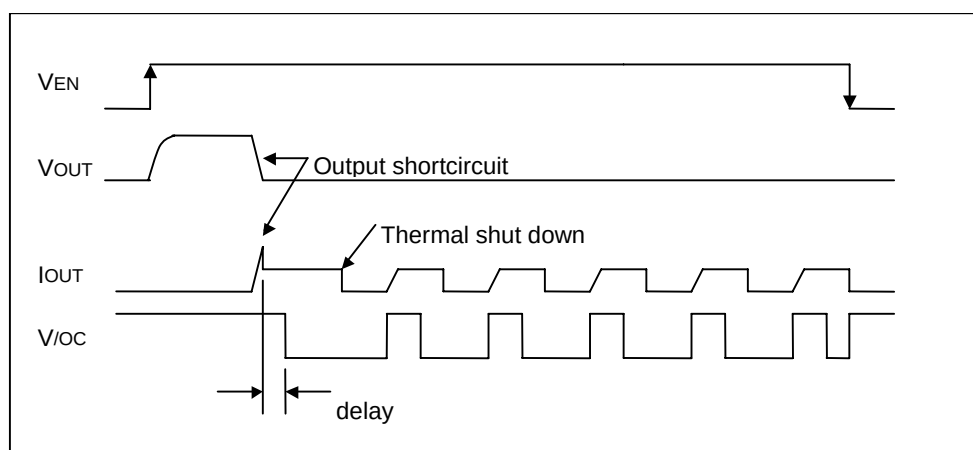
Figure 37. Over current detection, thermal shutdown timing (BD2055AFJ)
