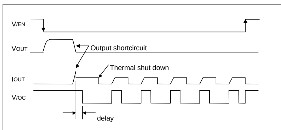
Figure 36. Over current detection, thermal shutdown timing (BD2045AFJ)
