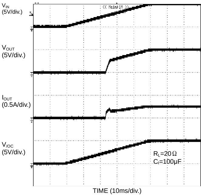
Figure 34. UVLO response Increasing V_{IN} (BD2045AFJ)
