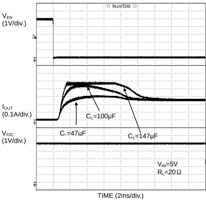
Figure 28. Inrush current response (BD2045AFJ)
