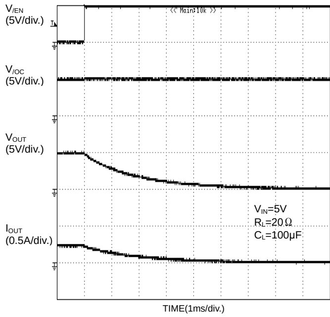
Figure 27. Output fall characteristic (BD2045AFJ)
