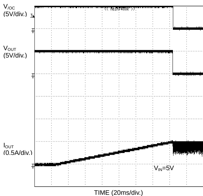
Figure 29. Over current response Ramped load (BD2045AFJ)
