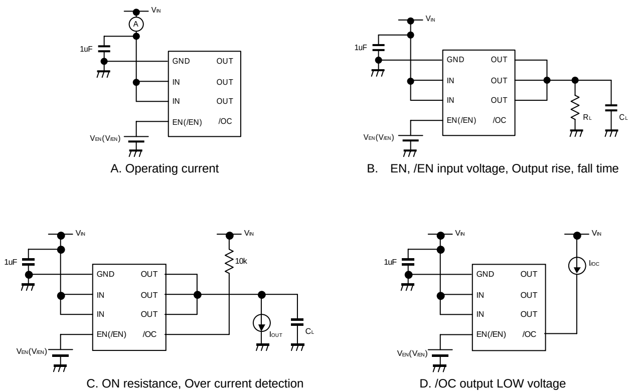
Figure 1. Measurement circuit
