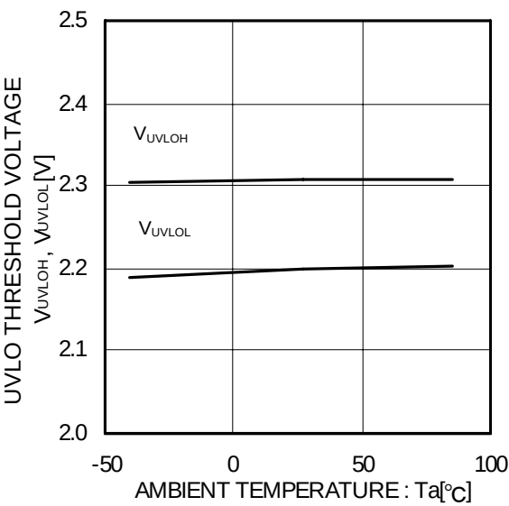
Figure 24. UVLO threshold voltage
