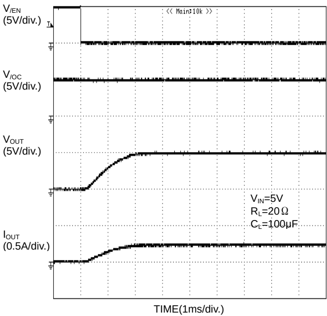
Figure 26. Output rise characteristic (BD2045AFJ)
