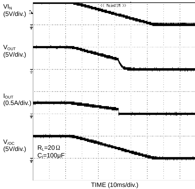
Figure 35. UVLO response Decreasing V_{IN} (BD2045AFJ)
