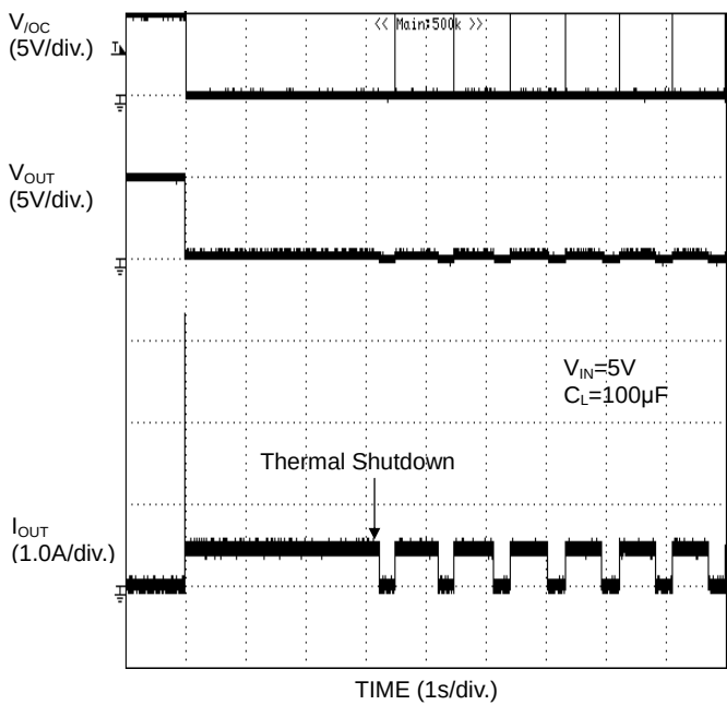
Figure 33. Over current response Enable to short-circuit (BD2045AFJ)
