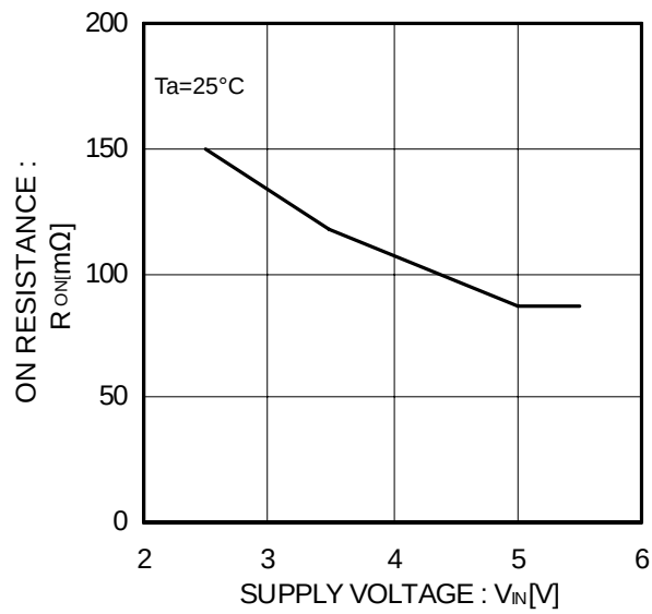
Figure 12. ON resistance
