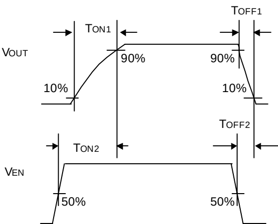
Figure 3. Timing diagram (BD2055AFJ)
