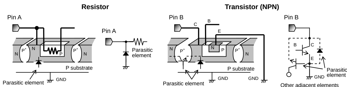
Figure 39. Example of monolithic IC structure
