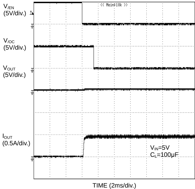
Figure 31. Over current response Enable to short-circuit (BD2045AFJ)
