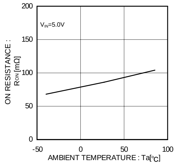
Figure 13. ON resistance
