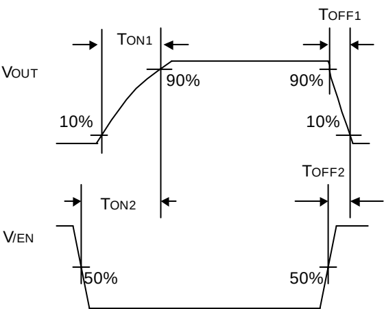
Figure 2. Timing diagram (BD2045AFJ)
