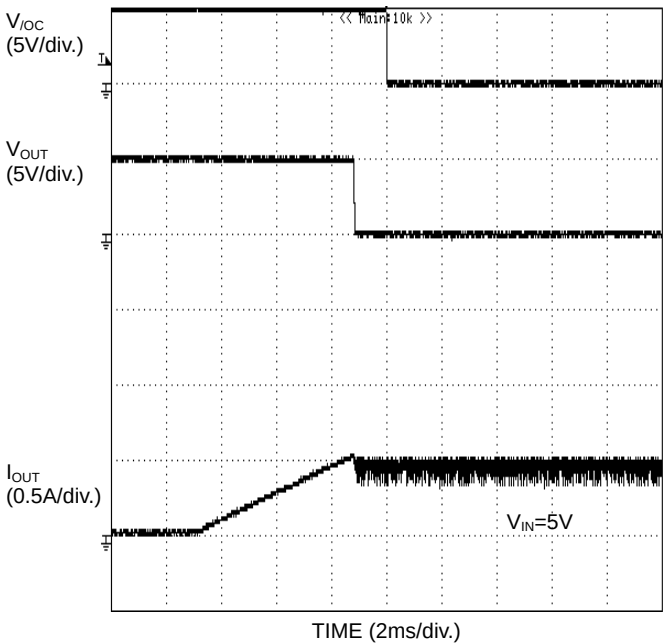
Figure 30. Over current response Ramped load (BD2045AFJ)
