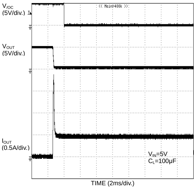
Figure 32. Over current response Enable to short-circuit (BD2045AFJ)
