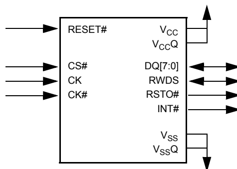
Figure 14.2 HyperBus Slave with Mandatory and Optional Signals
