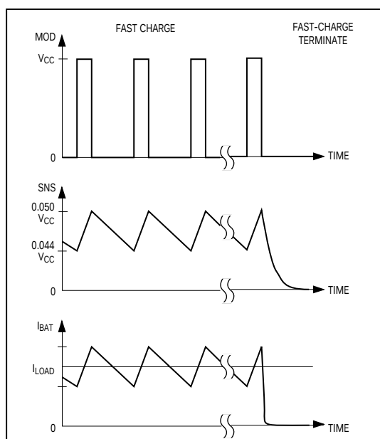
Figure 7. Current Regulation with an SNS Resistor
