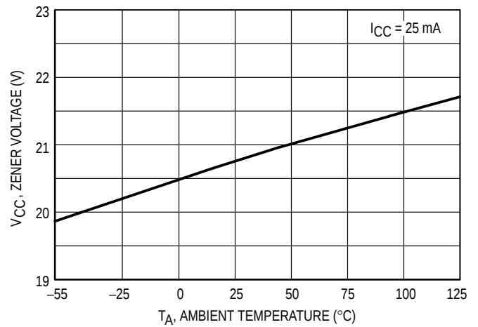
Figure 20. Power Supply Zener Voltage versus Temperature
