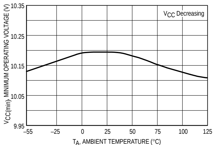
Figure 25. Minimum Operating Voltage After Turn-On versus Temperature
