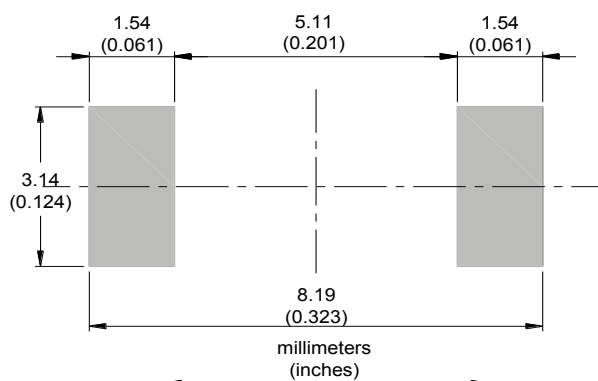
Figure 14. Footprint recommendation
